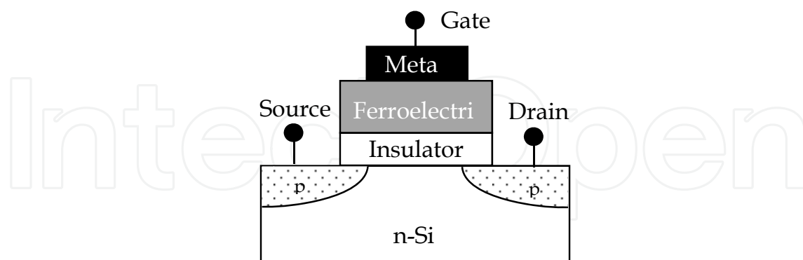
Fig. 1. Schematic of ferroelectric gate FET on n-Si substrate
