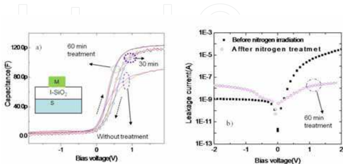
Fig. 7. Electronic properties of Pt/SiO 2 /Si MIS diodes with top electrode size of 7x10 4 μm 2 , a) C-V curves of MIS with with nitrogen treatment 60 min, 30 min and without the treatment, and b) I-V curves of MIS with 60 min and without nitrogen treatment.
