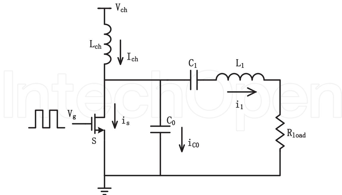
Fig. 2. Schematic of class E amplifier.
