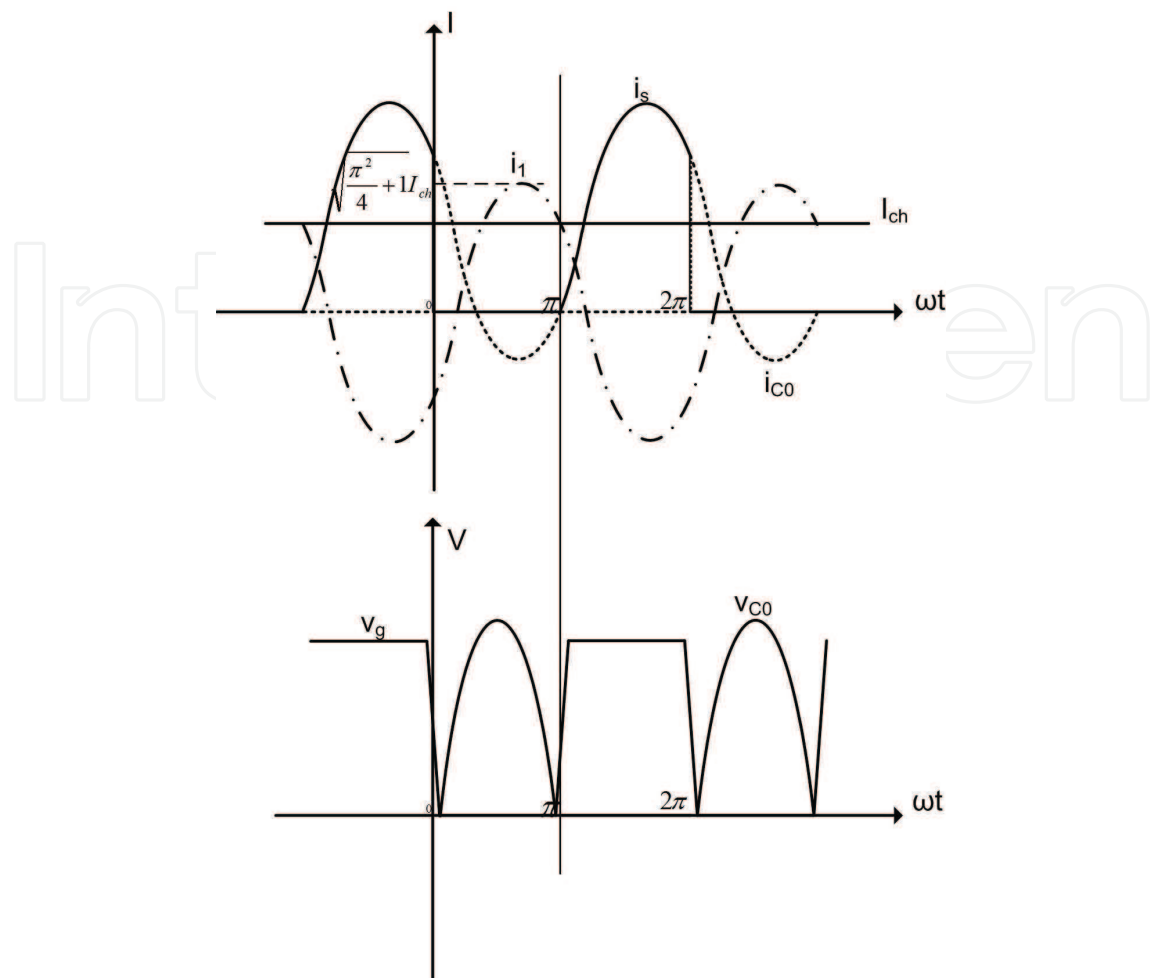
Fig. 3. Class E amplifier waveform when switch S has a 50% duty cycle and is turned on at time (2n + 1)\pi
