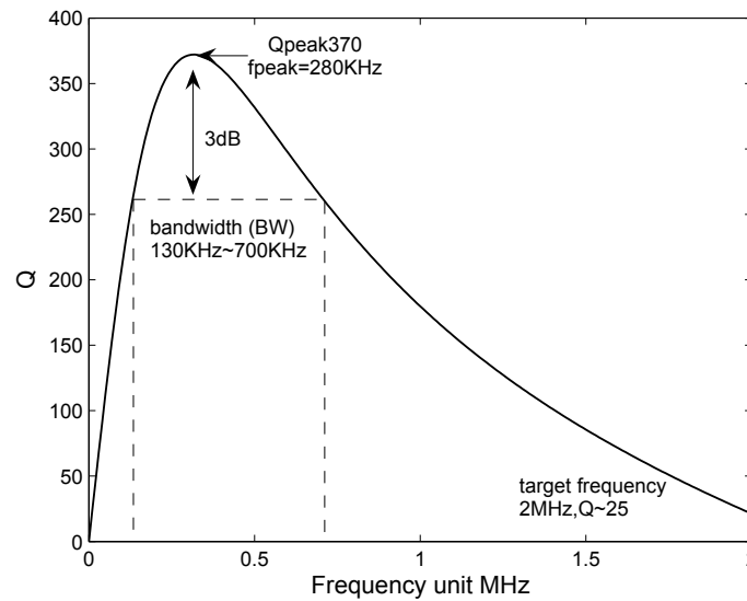
Fig. 9. Q vs Frequency curve. Coil specifications:
