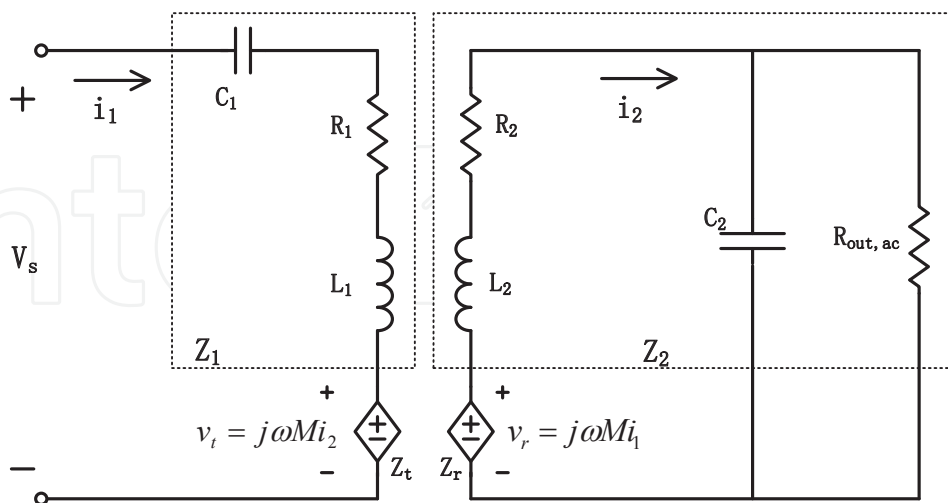
(b) Equivalent model as an ideal transformer
