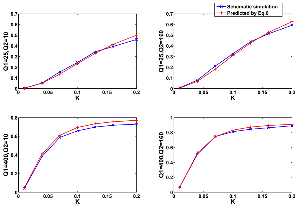
Fig. 6. Power efficiency with different coupling coefficient K
