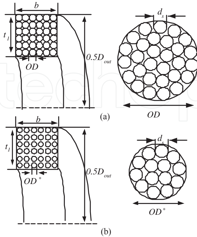
Fig. 14. Coils' cross sections. (a) Tightly wound litz coil with the maximum number of strands. (b) Loosely wound litz coil with less strands.
