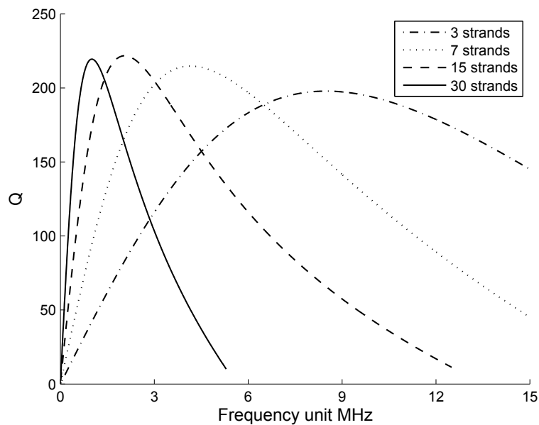
Fig. 15. Q vs Frequency curves for coils with the same cross sections but different numbers of strands.
