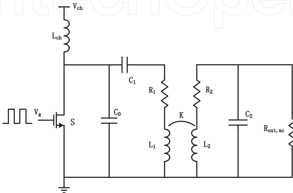
(a) Schematic of inductive power Link
