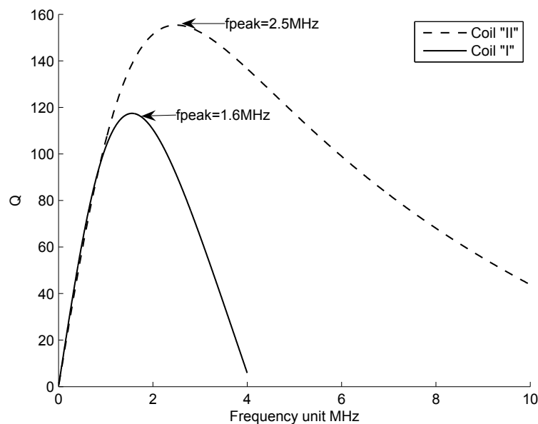
Fig. 12. Q vs Frequency curves of coil "I" and "II".
