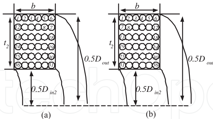
Fig. 13. Coils' cross sections. (a) Coil "II", loosely wound litz coil with normal winding sequence and separation between layers. (b) Coil "III", loosely wound litz coil with different winding sequence and separation between layers.
