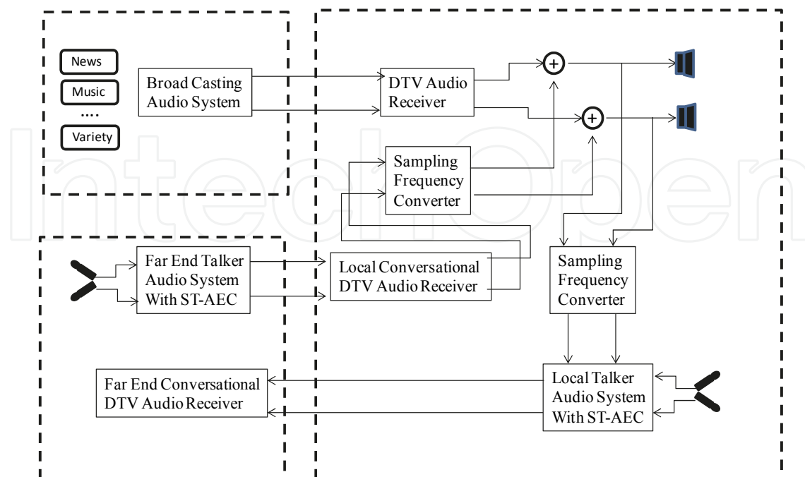
Fig. 1. Audio System Example in a Conversational DTV
