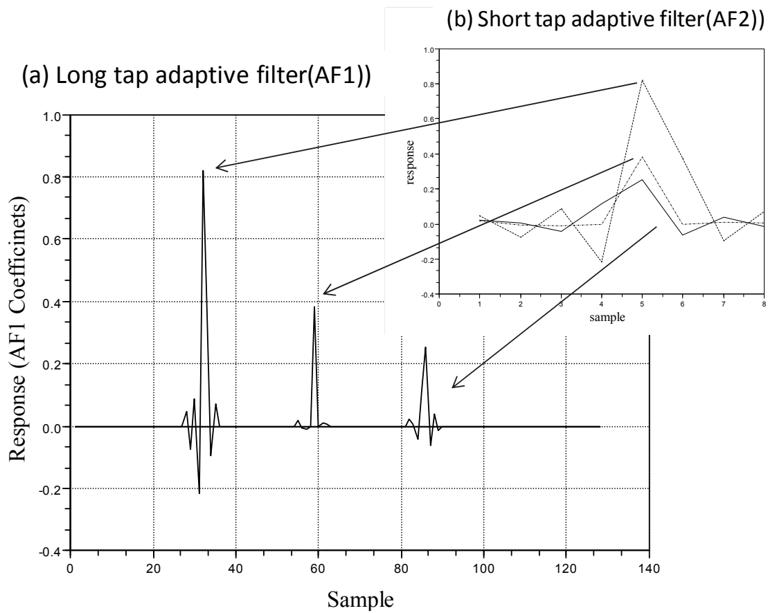
Fig. 11. Impulse Response Estimation Results in CCTF Block
