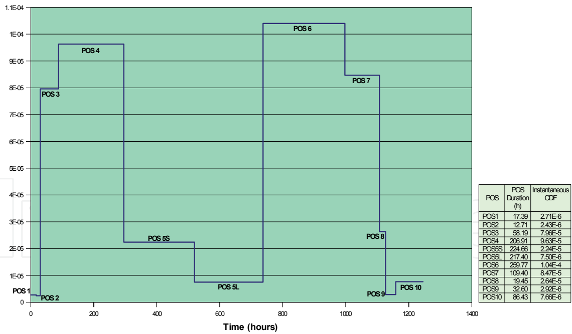
Fig. 3. Instantaneous CDF for each POS
