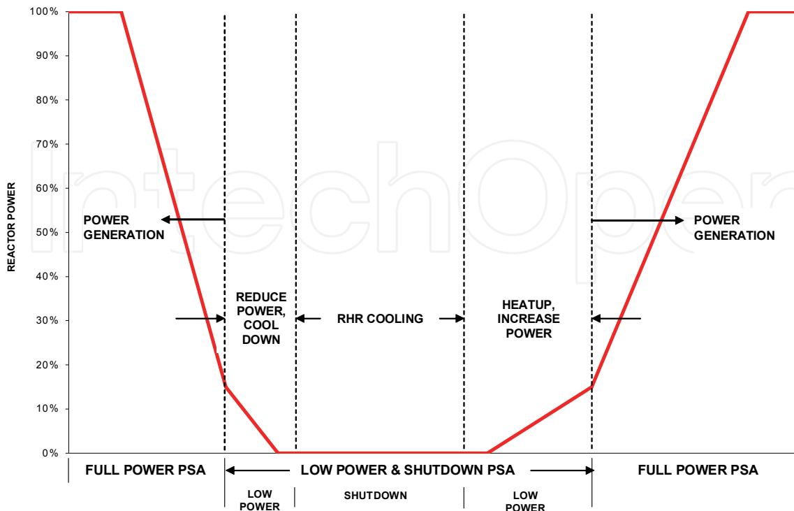
Fig. 1. Full power, low power and shutdown PSA
