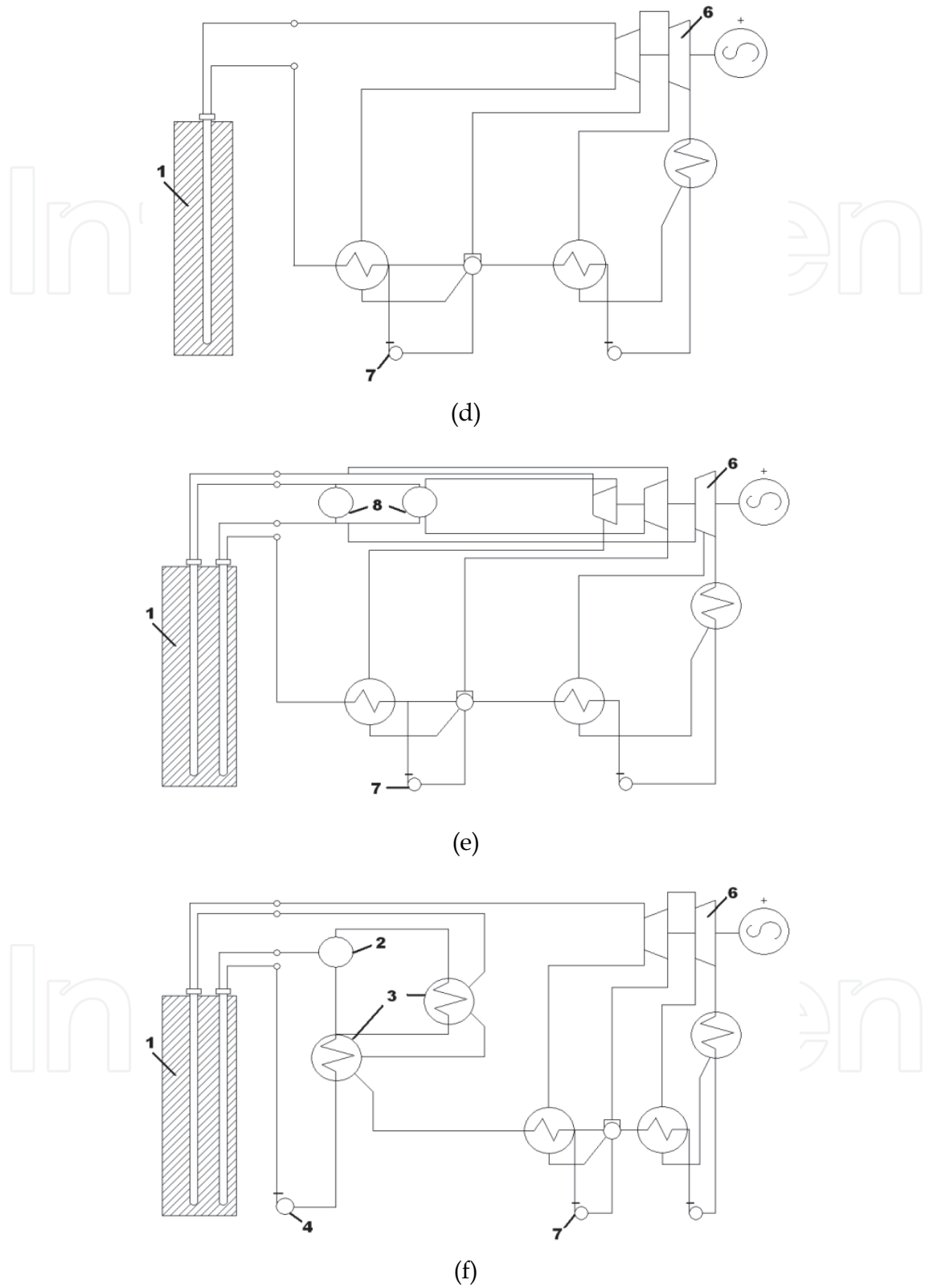
Fig. 3. Possible layouts of NPPs with steam reheat (Dollezhal et al. 1958): 1 – reactor; 2 – steam separator; 3 – SG; 4 – Main Circulation Pump (MCP); 5 – circulation pump; 6 – turbine with electrical generator; 7 – FWP; and 8 – intermediate-steam reheat.
