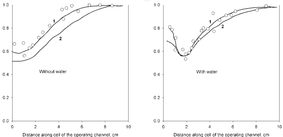
Fig. 6. Normalized thermal-neutrons-density distribution along cell of the operating channel (Dollezhall et al. 1958): 1 – experimental curve and 2 – design curve.
