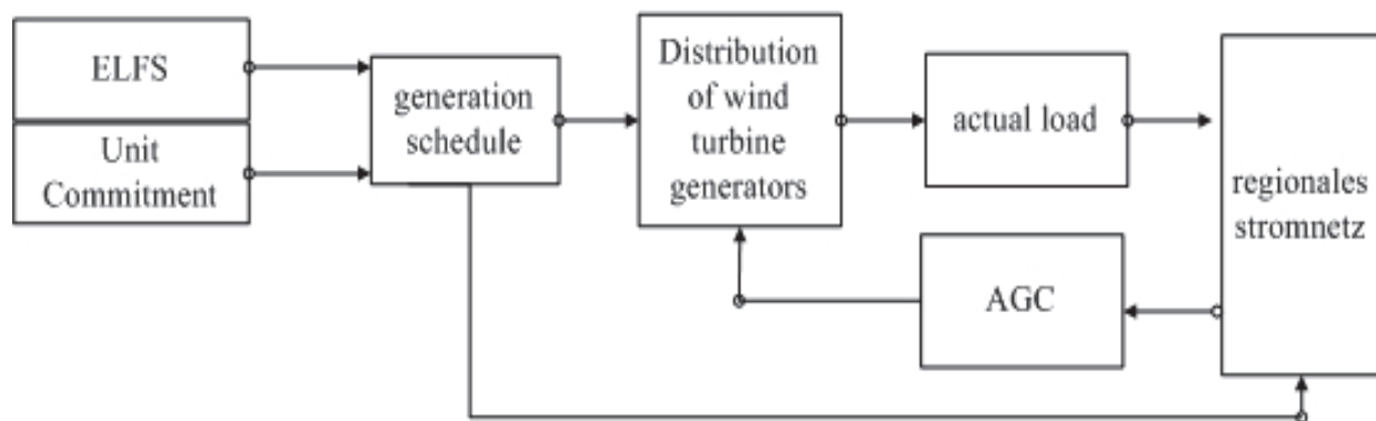
Fig. 15. Automatic generation control(AGC)
