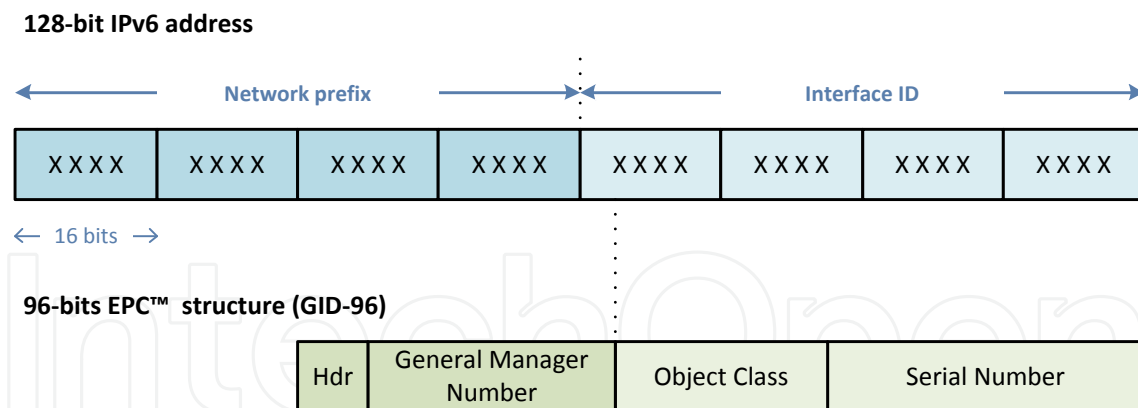
Fig. 5. IPv6-RFID address mapping with EPC™ GID-96.
