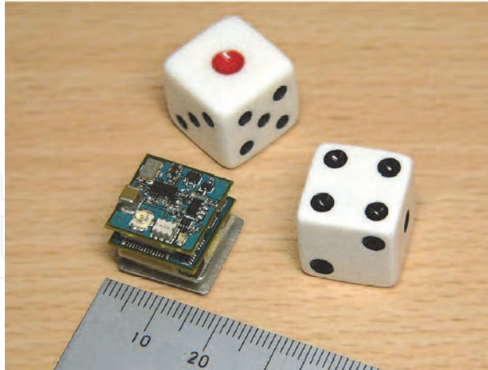
Fig. 4. A compacted active RFID tag
