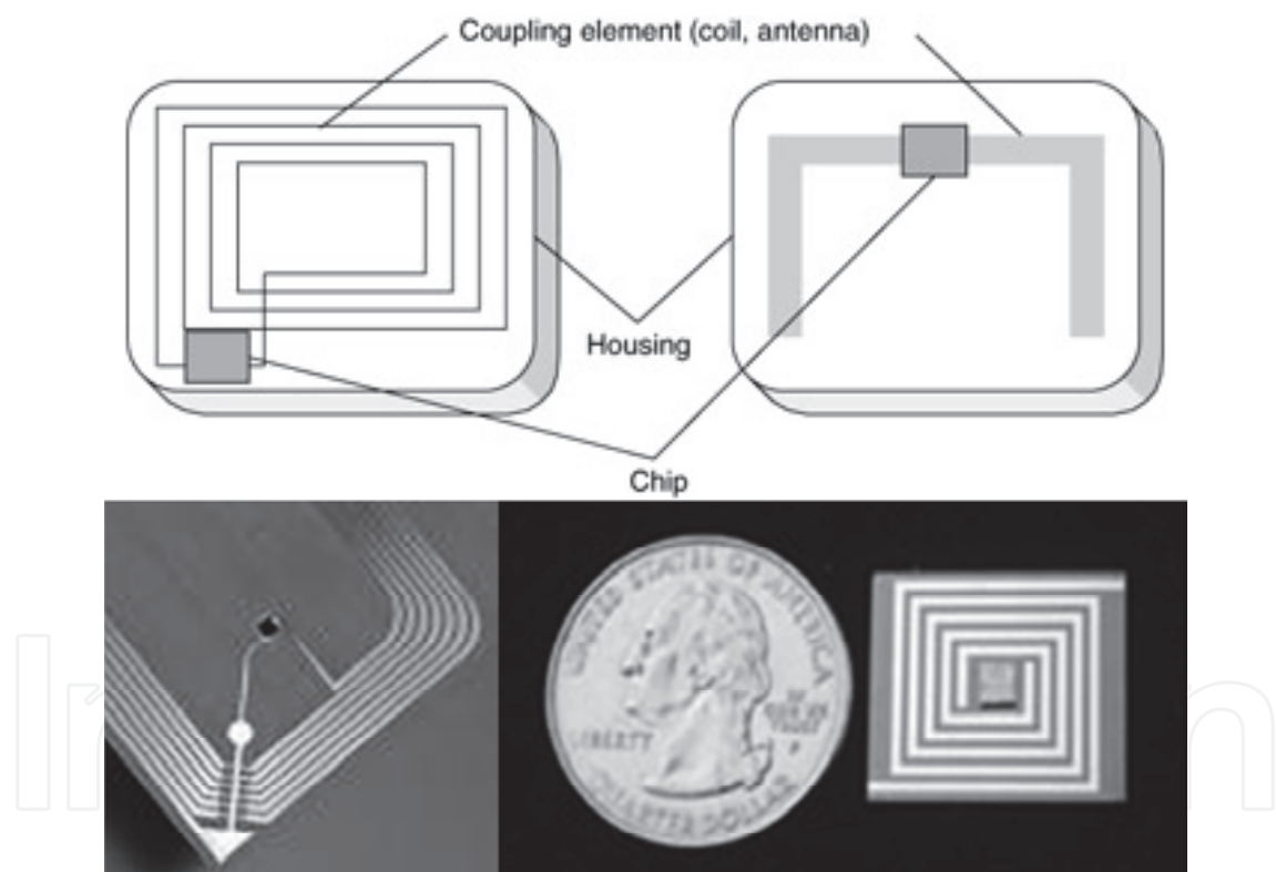
Fig. 2. The structure and outside view of RFID tags
