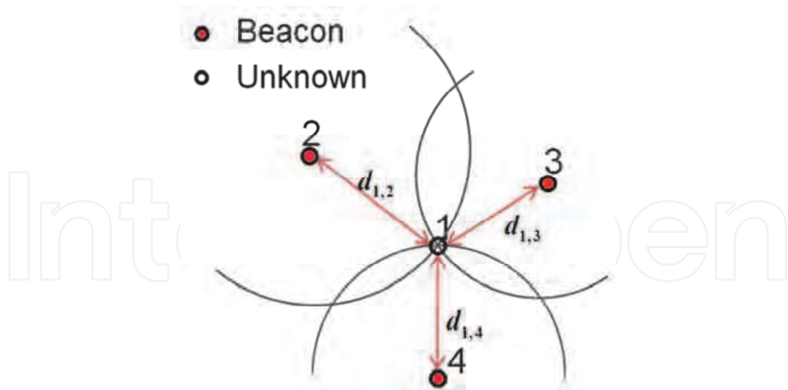
Fig. 6. The estimation of the position of an unknown node by using the trilateration method
