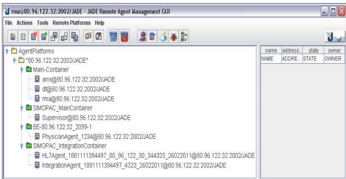
Fig. 4. Agents considered in SMA-SIMOPAC
