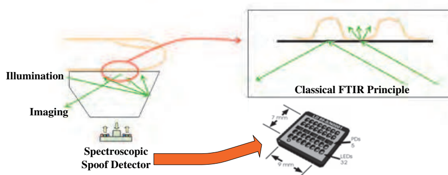
Fig. 5. FTIR and multispectral imager (Rowe, 2008).
