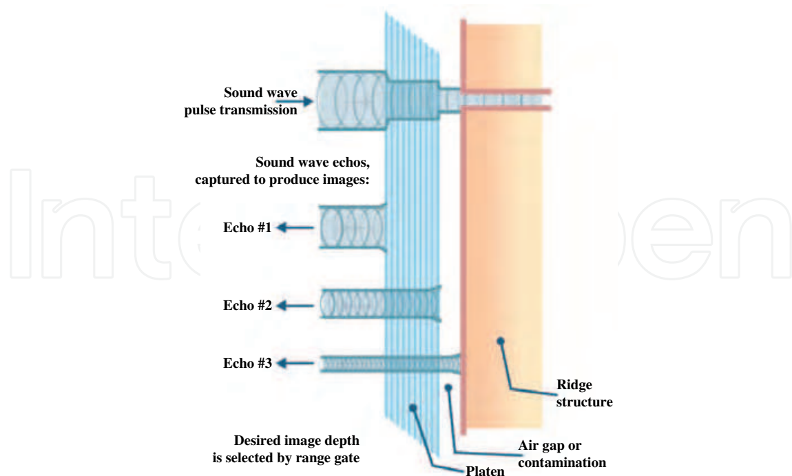
Fig. 7. Schematic of ultrasonic pulse/echo principle (UltraScan, 2004).
