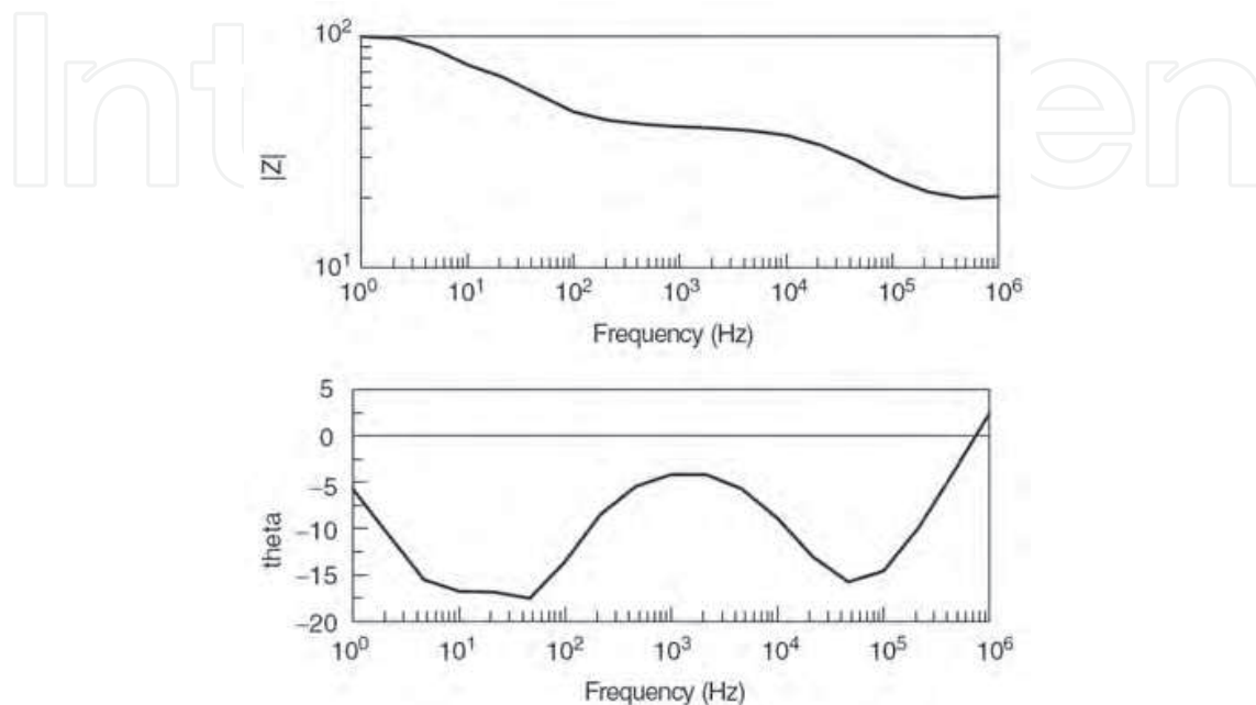
Fig. 12. Typical impedance spectrum obtained with four equal electrodes attached to the skin of the underarm (Grimmes et al., 2006).
