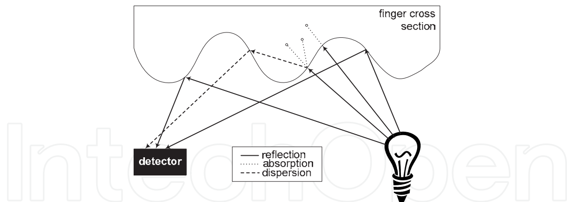
Fig. 13. Light absorption, dispersion and reflection by a fingerprint (Drahanský et al., 2006).
