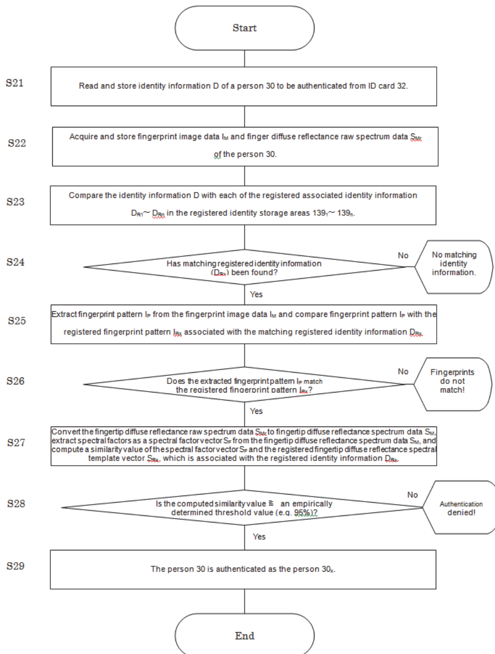
(Fig 8.b) Flowchart of a verification process
