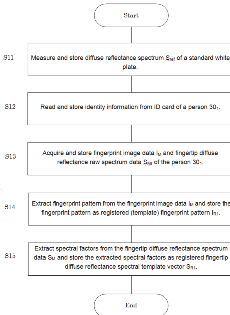
(Fig 8.a) Flowchart of an enrolment process
