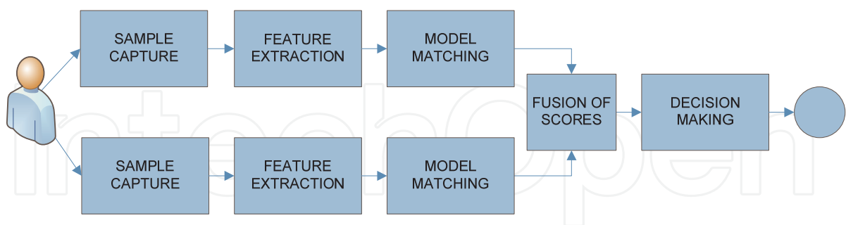
Fig. 9. Score level fusion.
