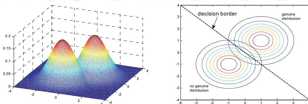
Fig. 15. Representation of two-dimensional Gaussian distribution scores.
