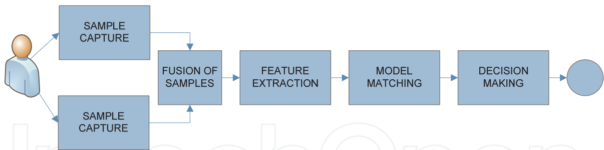
Fig. 7. Sample level fusion.
