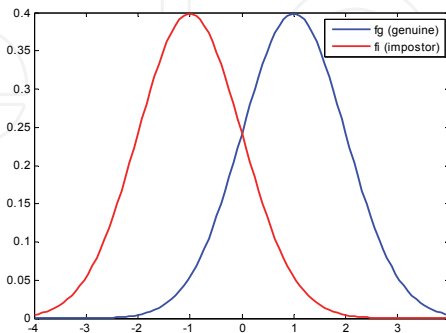
Fig. 14. Gaussian distribution of scores.
