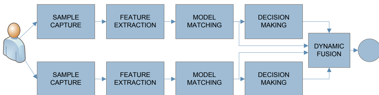
Fig. 11. Dynamic classifier selection.
