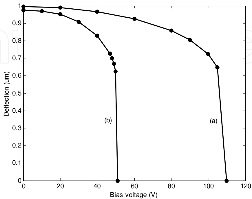
Fig. 9. Central deflection of a (curve a) clamped and (curve b) slotted diaphragm versus bias voltage
