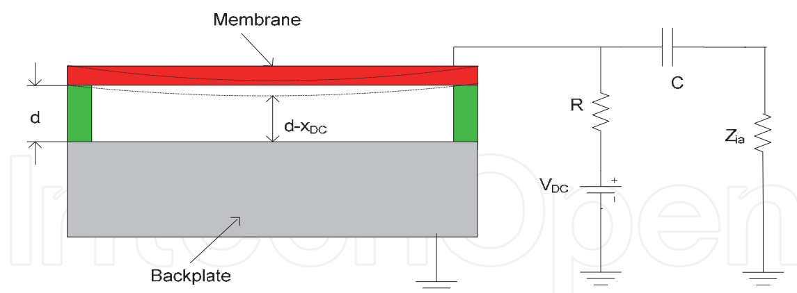
Fig. 1. Basic structure of the condenser microphone
