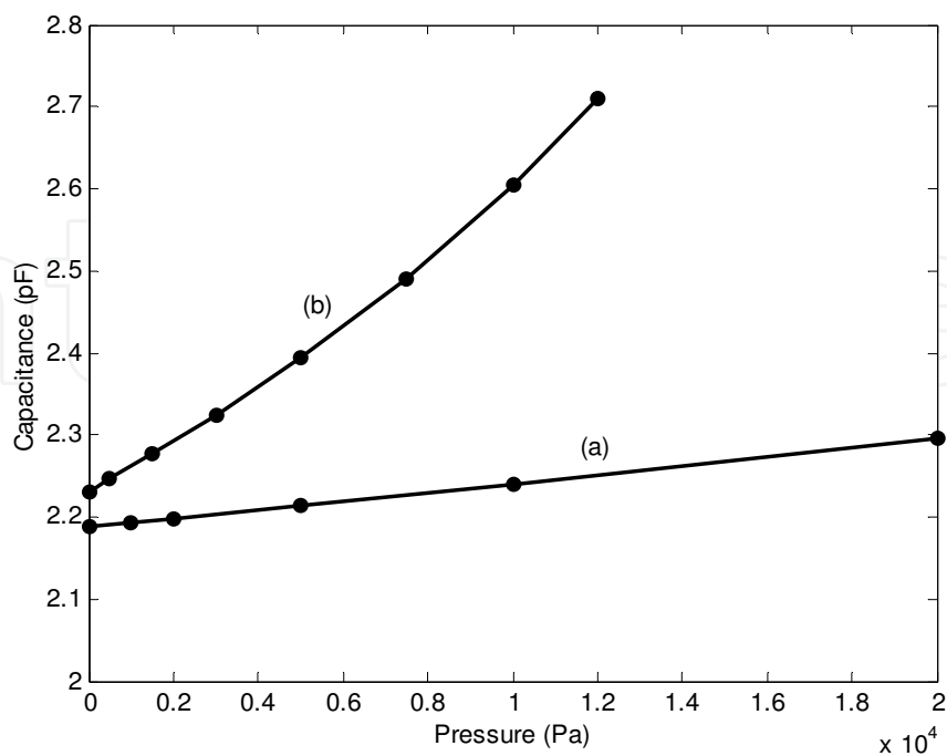
Fig. 10. Capacitance versus pressure for (a) the clamped and (b) the slotted microphones
