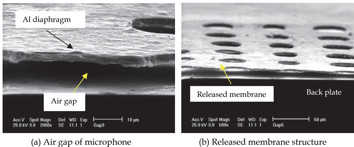
Fig. 15. Cross-section view of the microphone structure using SEM machine (Ganji and Majlis 2009)
