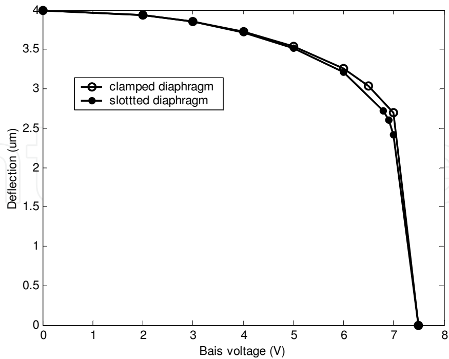
Fig. 7. Diaphragm deflection versus voltage
