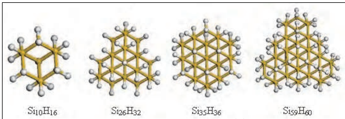
Fig. 3. Structures of \text{Si}_n\text{H}_m clusters represented in terms of ball-and-stick models. Yellow balls denote Si atoms and the white balls denote surface H atoms
