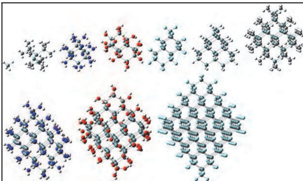
Fig. 6. Structures of Si-QDs embedded in an ionic environment, \text{SiO}_2 , \text{Si}_3\text{N}_4 , SiC matrix and a co-valent environment (left to right; top to bottom): \text{SiH}_4 , \text{Si}_5(\text{CH}_3)_{12} , \text{Si}_{10}(\text{NH}_2)_{16} , \text{Si}_{14}(\text{OH})_{20} , \text{Si}_{18}\text{F}_{24} , \text{Si}_{26}\text{H}_{32} , \text{Si}_{35}(\text{CH}_3)_{36} ; \text{Si}_{53}(\text{NH}_2)_{48} , \text{Si}_{84}(\text{OH})_{64} , \text{Si}_{165}\text{F}_{100}
