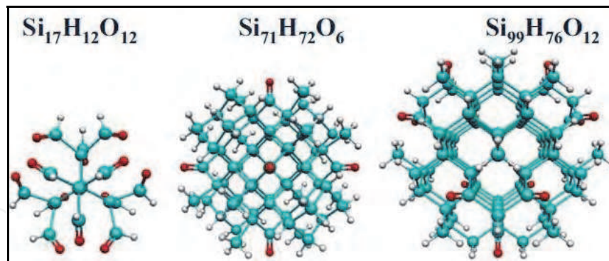
Fig. 5. Structure of oxidized nanocrystals with Td symmetry: The blue spheres are Si atoms, the red spheres are O atoms, and the white spheres are H atoms
