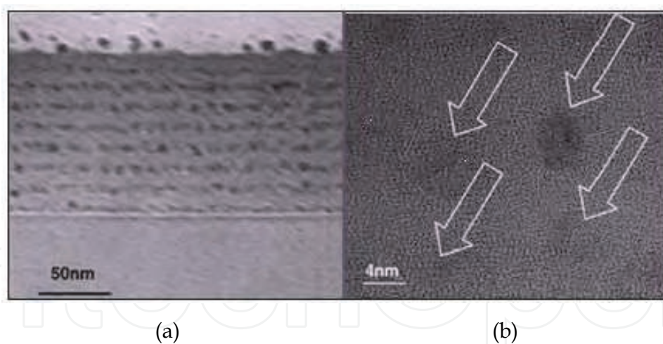
Fig. 1. Cross-sectional TEM (a) HRTEM (b) images of Si QDs in oxide. (a) Shows the layered structure and (b) shows individual nanocrystals in which crystal planes can be seen
