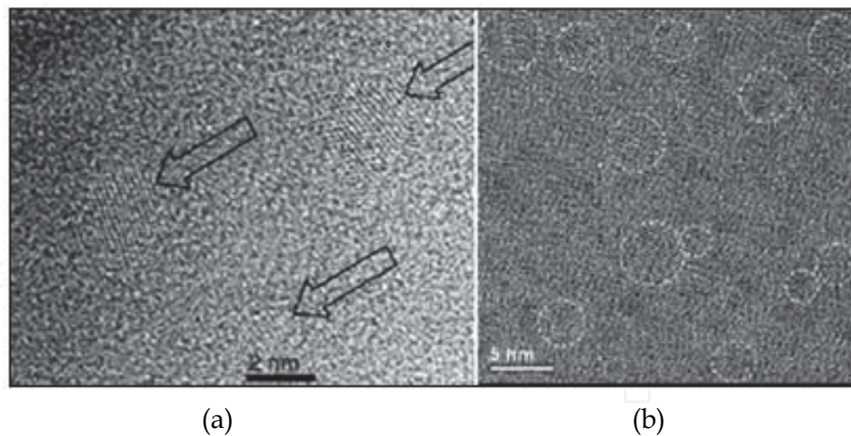
Fig. 2. HRTEM images of Si-QDs in (a) silicon nitride and (b) silicon carbide
