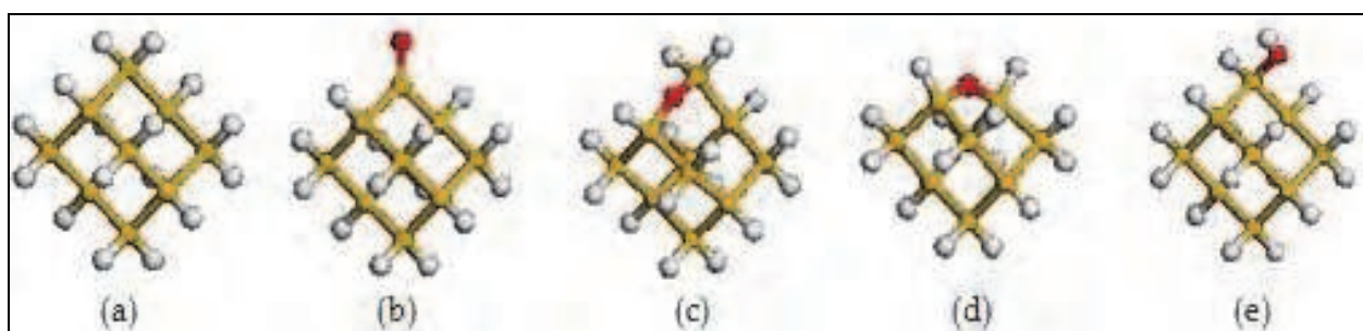
Fig. 4. Ball and stick representations of four possible oxygen passivation configurations, the yellow balls represent Si atoms, red balls represent O atoms, and the white balls, H atoms: (a) initial hydrogen-passivated silicon cluster, (b) double-bonded oxygen passivation configuration (c) backbonded (d) bridge-bonded (e) inserted oxygen configuration
