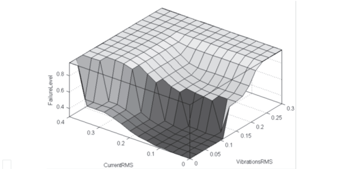
Fig. 17. Plotted surface showing the relationship between the system inputs Vibrations RMS value (g) and Stator Currents RMS value (A) versus the Failure Level output. (Motor speed: 1500 rpm, motor load: 0%)
