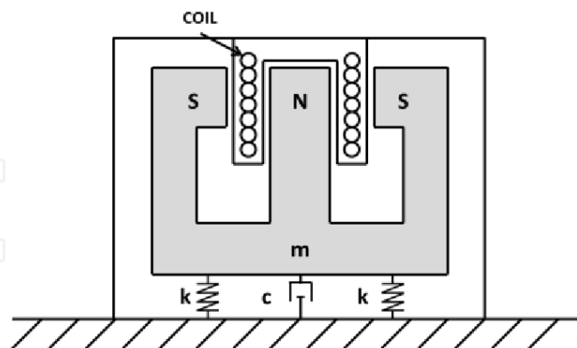
Fig. 8. Geophone reverse configuration scheme.
