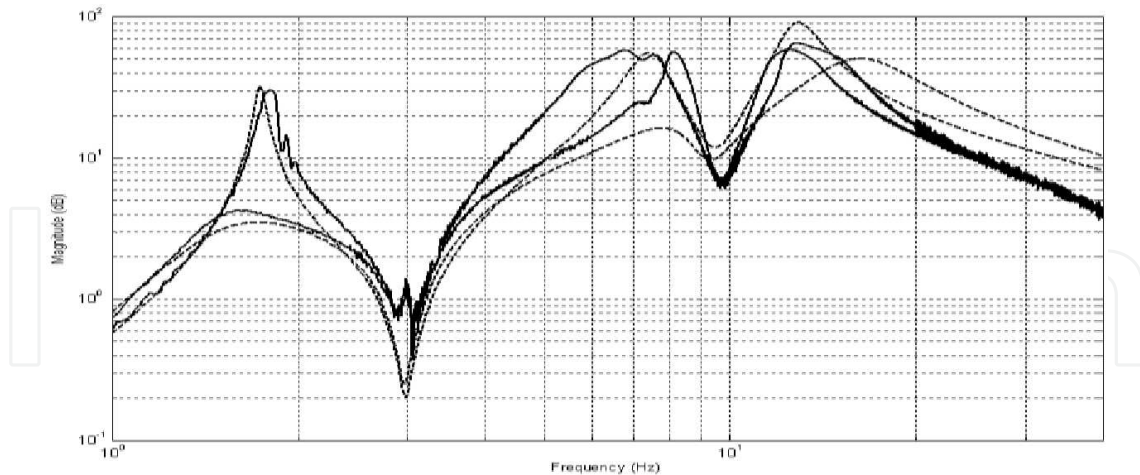
Fig. 17. Vibration damping action. Transfer function from the actuator force to the difference of frame and stage velocities ((\dot{q}_S - \dot{q}_F)/F_{ACT}) . Open-loop vs Closed-loop. Solid line: experimental; Dashed line: numerical.
