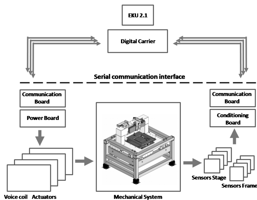
Fig. 10. Electronics subsystem.
