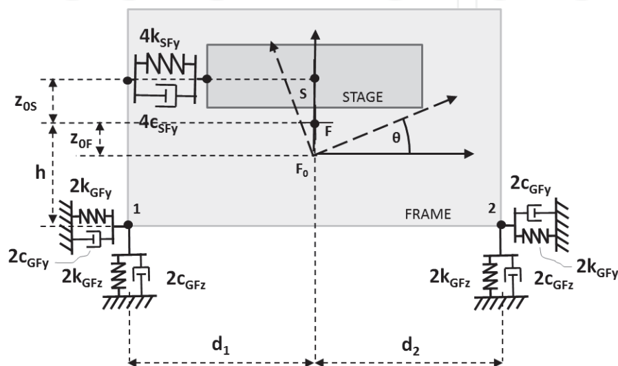
Fig. 14. YZ plane 4 dof model scheme.
