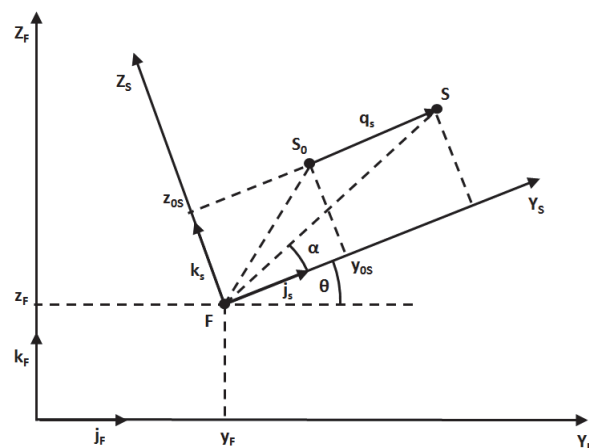
Fig. 13. YZ plane 4 dof kinematic relationships scheme.
