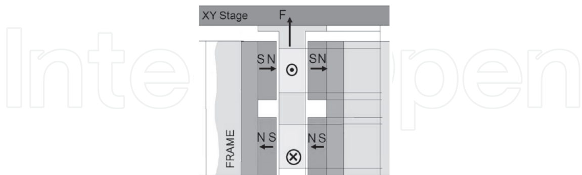
Fig. 5. Actuator force generation.
