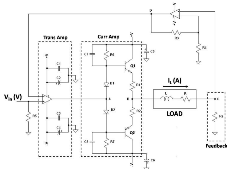
Fig. 12. Power electronic based on a trans-conductance amplifier.
