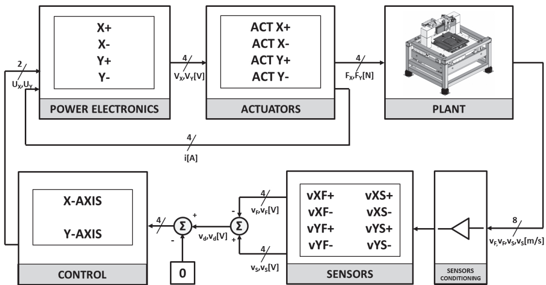
Fig. 3. Block diagram of the system.
