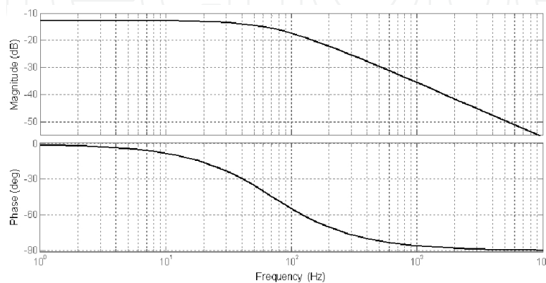
Fig. 6. Actuator trans-conductance transfer function (magnitude and phase).
