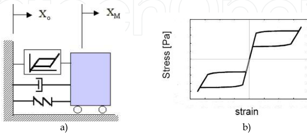
Fig. 19. a) Equivalent mechanical model of the SDOF scaled structure b) The hysteresis /energy dissipation behavior of the re-centering device
