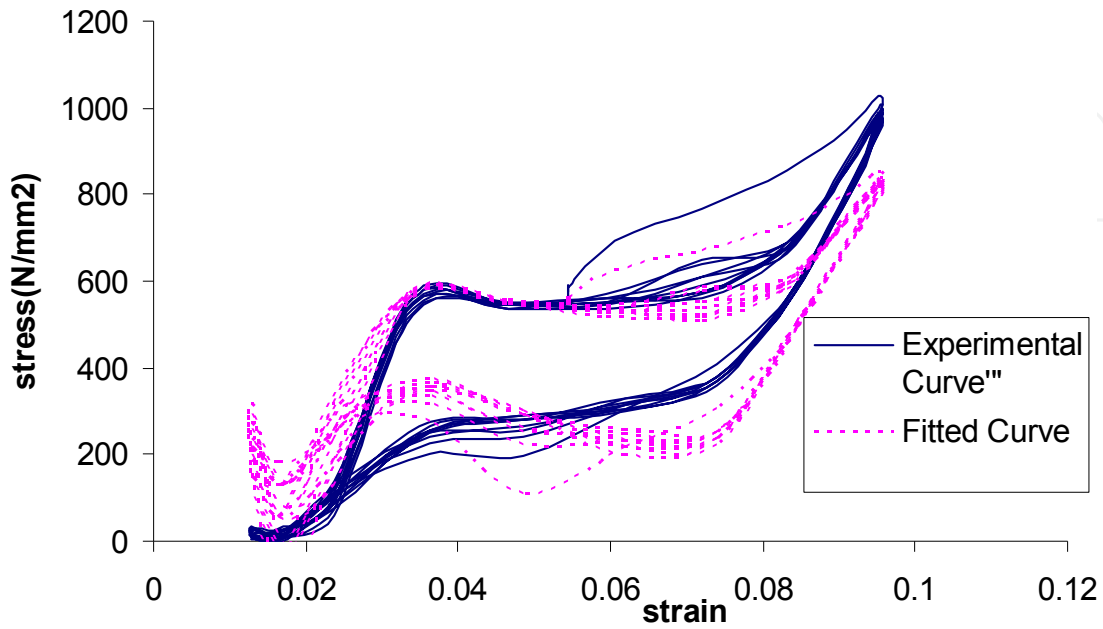
Fig. 15. Cyclic behaviour of prestrained wires –maximum energy dissipation obtained and the fitted curve.
