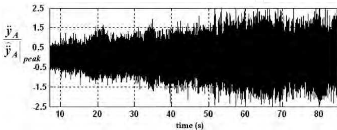
(a) acceleration at attachment point A of ATVA, normalised with respect to \bar{y}_A|_{peak} (defined in Figure 24)
