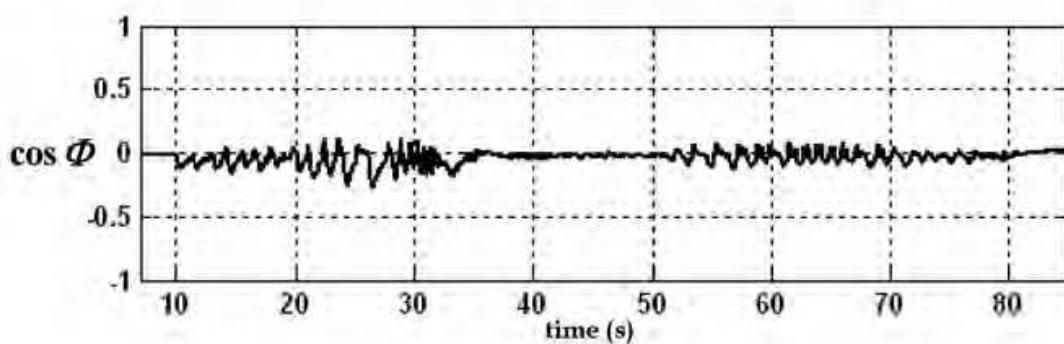
(b) cosine of phase shift \Phi between \ddot{y}_g and \ddot{y}_A
