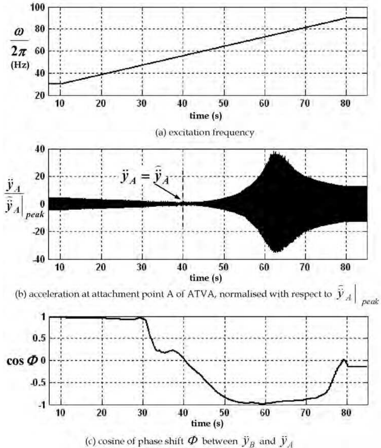
Fig. 24. Swept-sine test with controller turned off and ATVA tuned to a fixed frequency of 56 Hz ( \hat{\ddot{y}}_A|_{peak} is the amplitude of \hat{\ddot{y}}_A , the tuned acceleration at A at an excitation frequency of 56 Hz)
