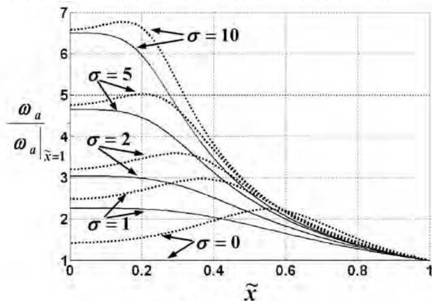
(a) Tuned frequency characteristics
