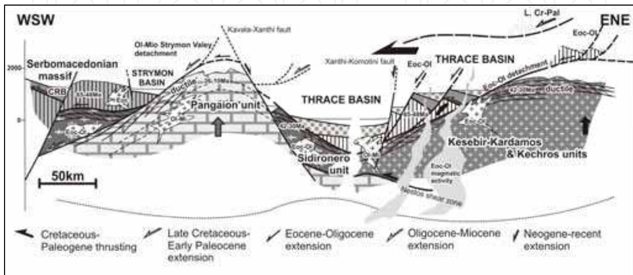
Fig. 9. Geometry of kinematics during Paleogene-Neogene extension of Rhodope Massif and formation of the Paleogene volcano-sedimentary Thracian basin on top of the Paleogene extensional detachment fault system, simultaneously with uplift of deep crustal metamorphic Rhodope units. Extension migrates towards SW-SSW. Legend as in Fig. 2
