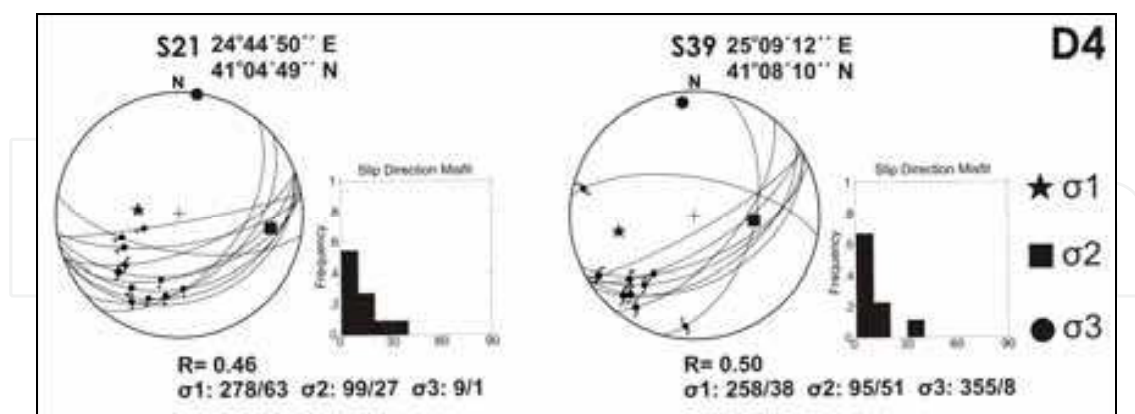
Fig. 16. Faults–striae data and deduced paleostress field ( \sigma_1 > \sigma_2 > \sigma_3 ) orientation during D4 (equal area, lower hemisphere). Fluctuation histograms of deviation angles (angle between the calculated slip vector and the measured slickenside) and stress ratio R = \sigma_2 - \sigma_3 / \sigma_1 - \sigma_3 are shown. The geographic coordinates for each station are also indicated
