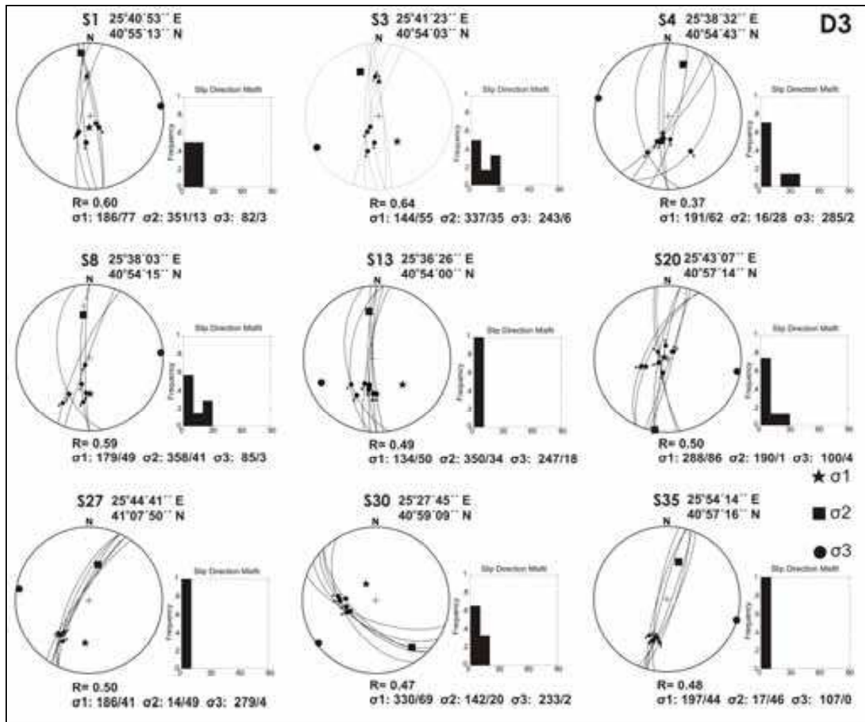
Fig. 15. Faults-striae data and deduced paleostress field ( \sigma_1 > \sigma_2 > \sigma_3 ) orientation during D3 (equal area, lower hemisphere). Fluctuation histograms of deviation angles (angle between the calculated slip vector and the measured slickenside) and stress ratio R = \sigma_2 - \sigma_3 / \sigma_1 - \sigma_3 are shown. The geographic coordinates for each station are also indicated
