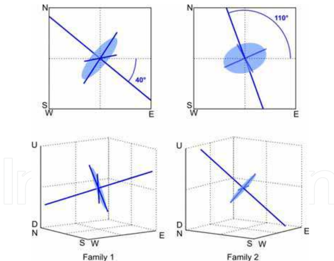
Fig. 14. Map views (up) and 3-D views (down) of the crack source mechanism obtained for the two families of LP events. The circular areas represent the cracks, the normalized eigenvectors are represented by solid lines, and the longest of these are the normal cracks. A subvertical dike striking SSW-NNE is obtained for family 1, and a crack striking SW-NE that lies on a plane inclined of 45^\circ is computed for family 2. Redrawn from De Barros et al. (2011)
