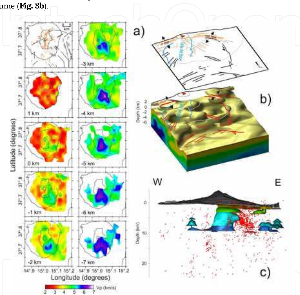
Fig. 3. (a) Mt. Etna's V_p velocity model (Patanè et al. 2006), between 1 a.s.l. and 7 km b.s.l., in the well-resolved regions of the model. The gray lines are elevation isolines (every 1000 m). In the top left square the historical eruptive fissures (orange lines) and major faults (black lines) are shown. (b) Isosurface image at V_p of 3.5 km/s for the central-eastern and northern sectors of the volcano. A complex pattern of solidified magma chambers and conduits with variable dimensions is recognizable. At the top, historical eruptive fissures (orange lines) and major faults (black lines) are shown. Major faults are also projected in red in the 3D block. (c) Cumulative isosurfaces for different velocities V_p showing the 3D geometry of the HVB down to 10 km depth. The seismicity occurring during 2001-2003 is also shown (red dots), evidencing how the HVB is almost an aseismic volume surrounded by an active seismic region
