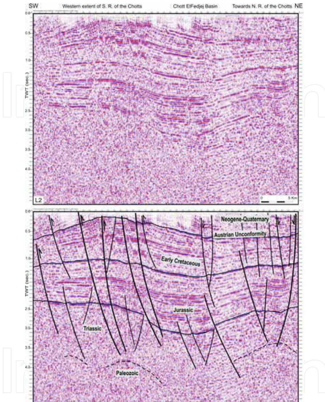
Fig. 5. Seismic section L2 of the Chott El Fedjaj, showing two positive flower fault structures trending east-west and evolution of Mesozoic series under faulting change and halokinesis of northern and southern range of the Chotts
