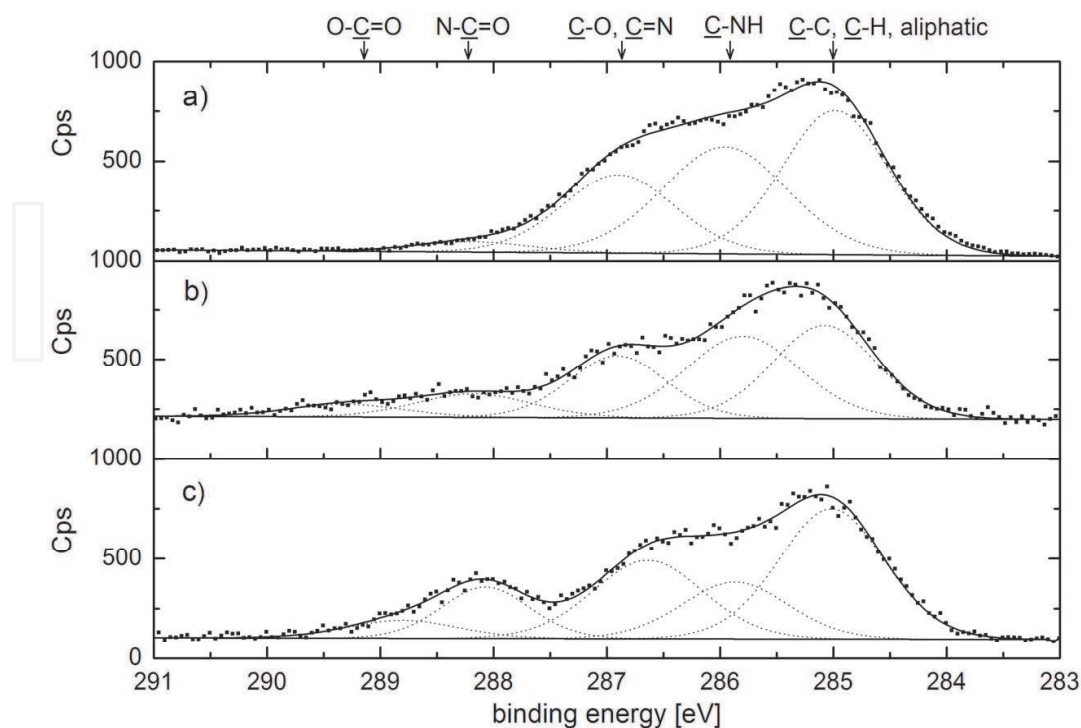
Fig. 9. High-resolution XPS-analysis of C1s spectra of PPAAm (a), the immobilization of polyethylene glycol diacid (PEG DA, b) in the first and the following coupling of collagen I (COL, c) in the second step.
