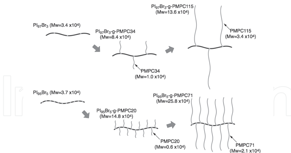
Fig. 4. Schematic representation of PIBr and PIBr-g-PMPC. (Reproduced from Iwasaki et al., (2004) Macromolecules , Vol. 37, No. 20, pp. 7637-7642, Copyright (2004), with permission from the American Chemical Society)
