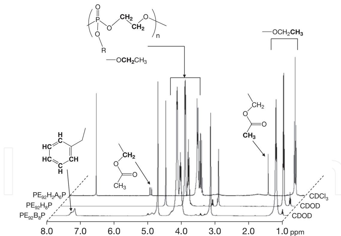
Fig. 14. ^1\text{H} NMR spectra of polyphosphoester bearing acetoxymethyl ester groups and the prepolymers.
