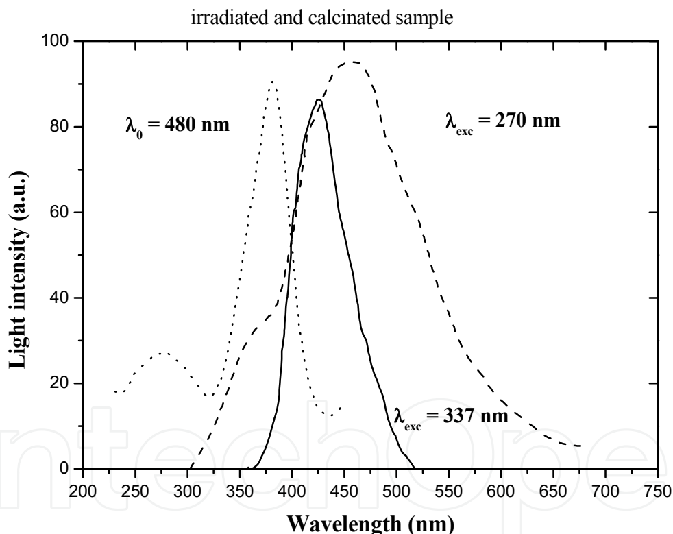
Fig. 6. Excitation spectrum of the intrinsic emission of polycrystalline ZrO_2 at RT described by dotted line (....). PL emission spectra of polycrystalline ZrO_2 powder samples for excitation wavelength of 270 nm described by dashed line (---). PL emission spectra of polycrystalline ZrO_2 powder samples for excitation wavelength of 337 nm described by solid line (—) beta-irradiated samples.
