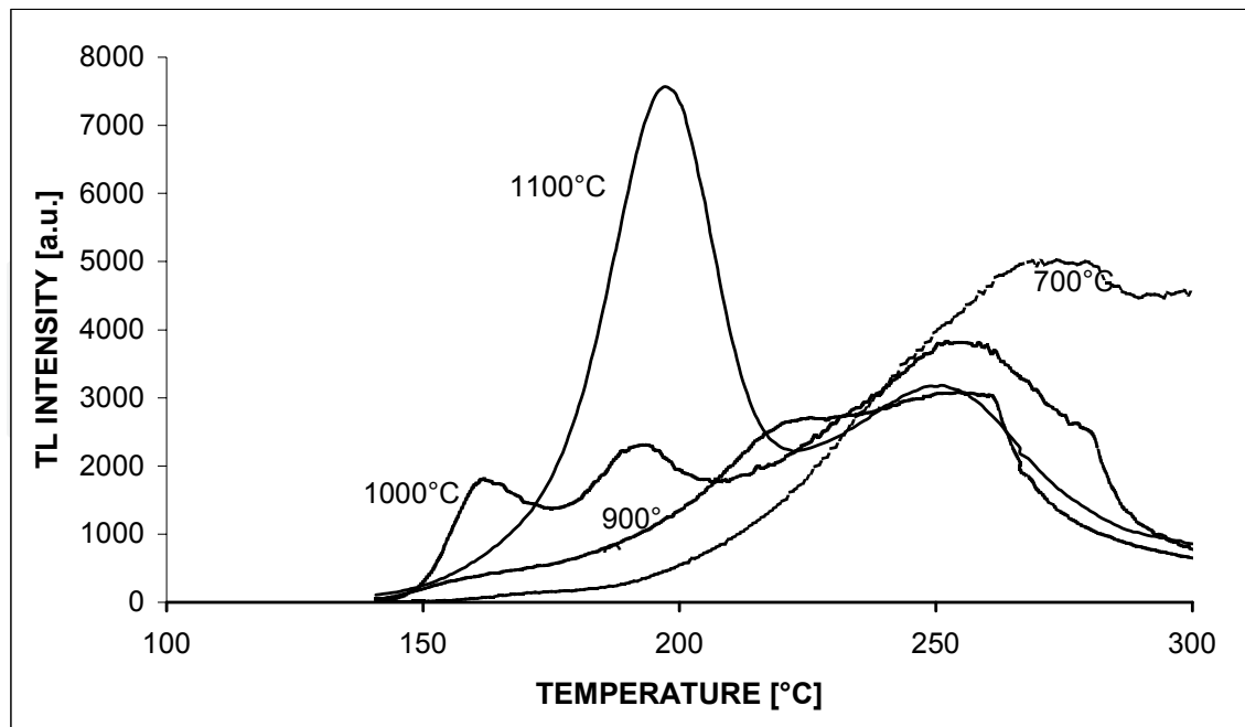
Fig. 2. TL glow curves of ZrO_2 after crystallization treatment process.
