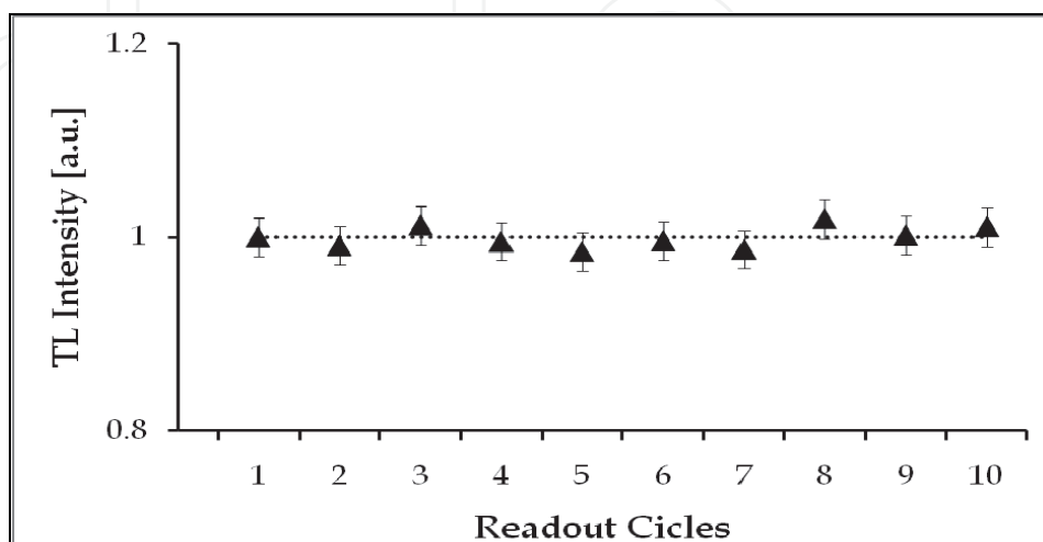
Fig. 10. Reproducibility of polycrystalline ZrO_2 powder
