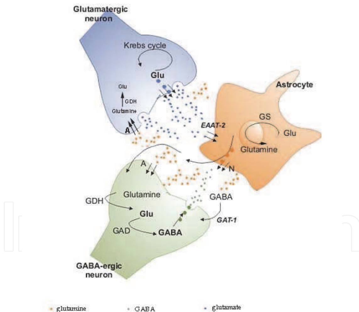
Fig. 2. The schematic presentation of glutamatergic-GABAergic transformation involving the pyramidal neuron, GABAergic interneuron and astrocyte. Glu-glutamate; GABA- \gamma amino butyric acid; GS-glutamine synthetase; GAD-glutamate decarboxylase; GDH-glutamine dehydrogenase; GAT-1-GABAergic transporter 1; EAAT-2-excitatory amino acid transporter 2; A-system A transporters; N-system N transporters
