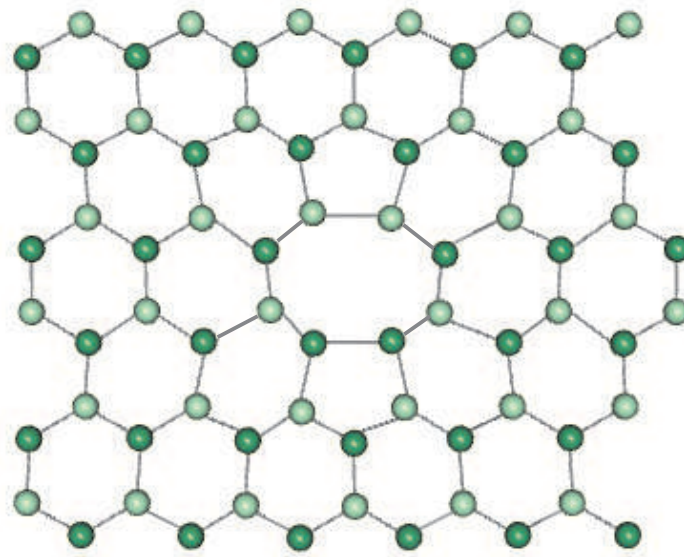
Fig. 3. Pentagon-octagon-pentagon divacancy.
