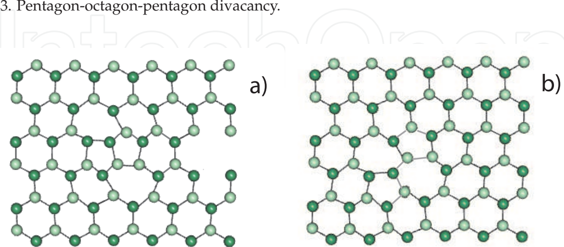
Fig. 4. (a) Stable 7-5-5-7 defect. (b) Unstable 5-7-7-5 Stone Wales defect.
