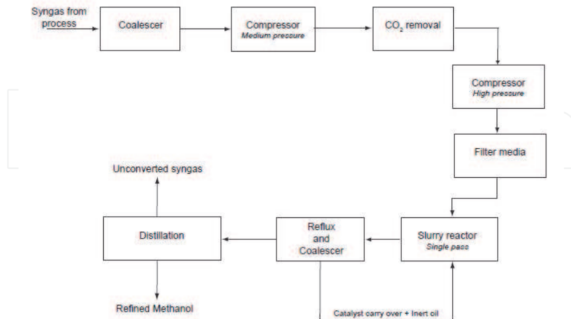
Fig. 5. Enkern Inc. liquid phase methanol process
