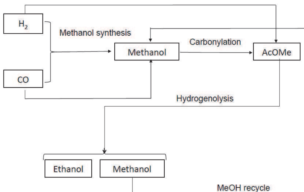
Fig. 6. Enerkem Inc. ethanol pathway production.
