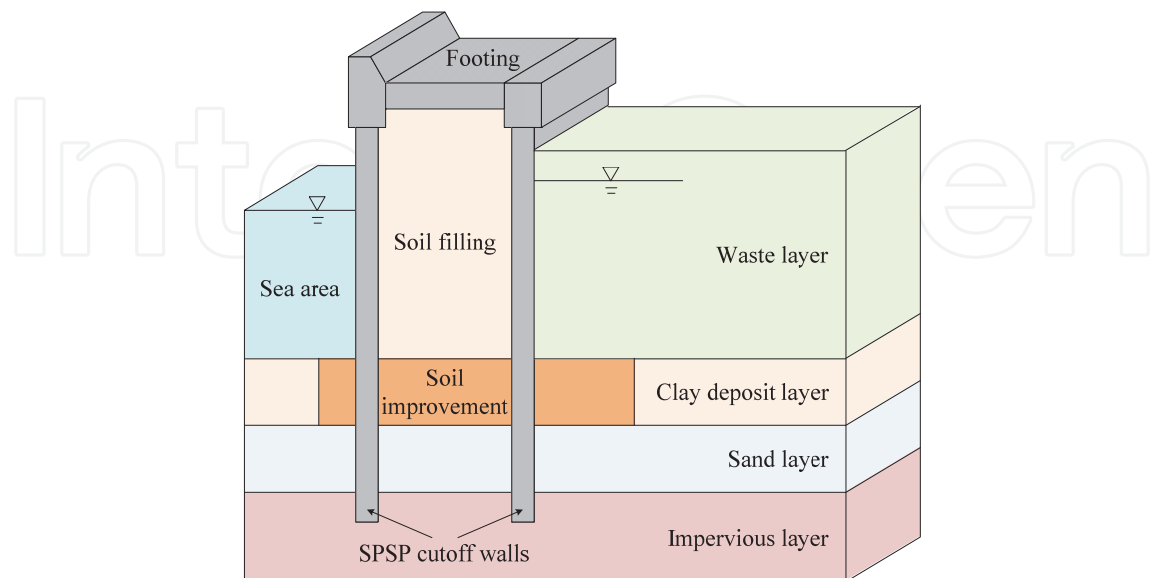
Fig. 6. Overview of vertical and bottom cutoff barriers generally constructing at coastal landfill sites
