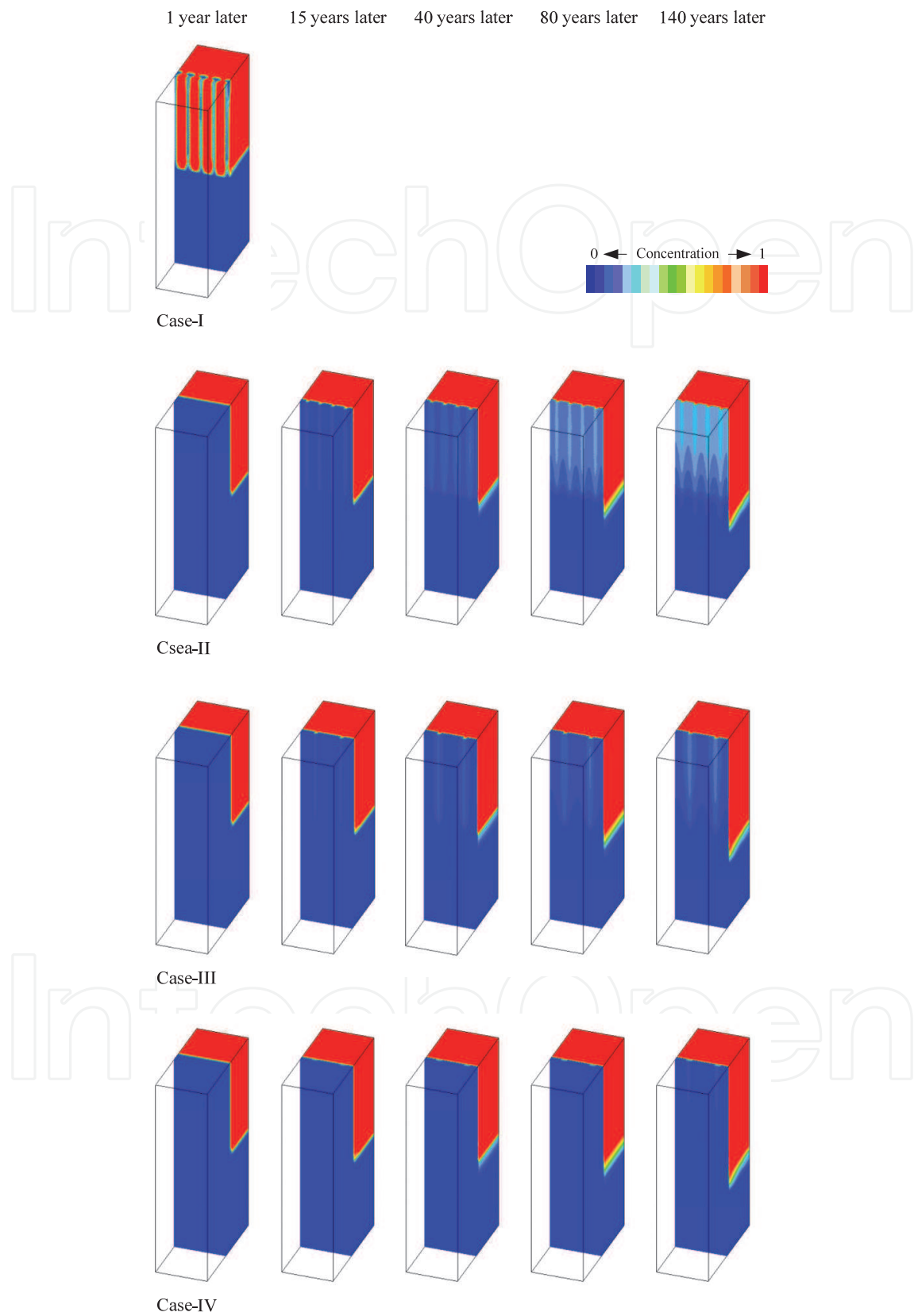
Fig. 16. Distribution of concentration of toxic substances leaking out from waste layer in Case-I to Case-IV
