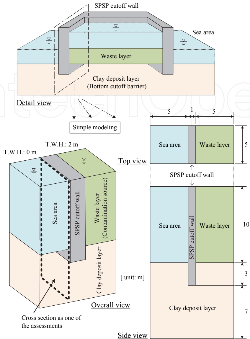
Fig. 5. Three-dimensional cross section of landfill site assumed as a basic case in the analysis the coastal landfill site is considered for setting the three-dimensional cross-section. At the bottom of the waste layer as well as in the sea bed, a clay deposit layer is assumed to exist, and this layer fulfils the role as a bottom cutoff barrier in the coastal landfill site. The SPSP cutoff wall is penetrated upto a depth of 3 m in the clay deposit layer, and the hydraulic conductivity of the SPSP cutoff wall is varied to provide different examination cases. In the construction of the SPSP cutoff wall at coastal landfill sites, double SPSP cutoff walls may be used due to ensure mechanical stability and fail-safe concept of landfill sites, as shown in the overview in Fig. 6. Furthermore, the clay deposit layer may be improved by sand compaction pile (SCP) methods in order to enhance the mechanical stability of the SPSP cutoff walls (Waterfront Vitalization and Environment Research Center, 2002). However, the main objective of this study is the evaluation of the environmental feasibility (containment effect of leachate containing toxic substances) of the SPSP cutoff wall. Therefore, the coastal landfill site is simplified, as shown in Fig. 5, as a three-dimensional cross-section that comprises a single SPSP cutoff wall, waste layer and clay deposit layer.
