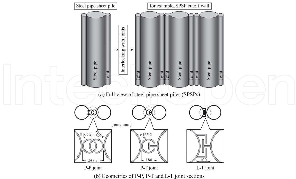
Fig. 2. Schematic diagram of steel pipe sheet piles with joint sections
