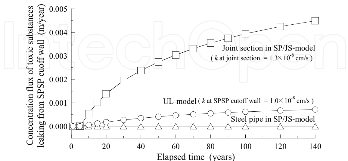
Fig. 8. Concentration flux of toxic substances leaking from SPSP cutoff wall on sea side with elapsed time for both models
