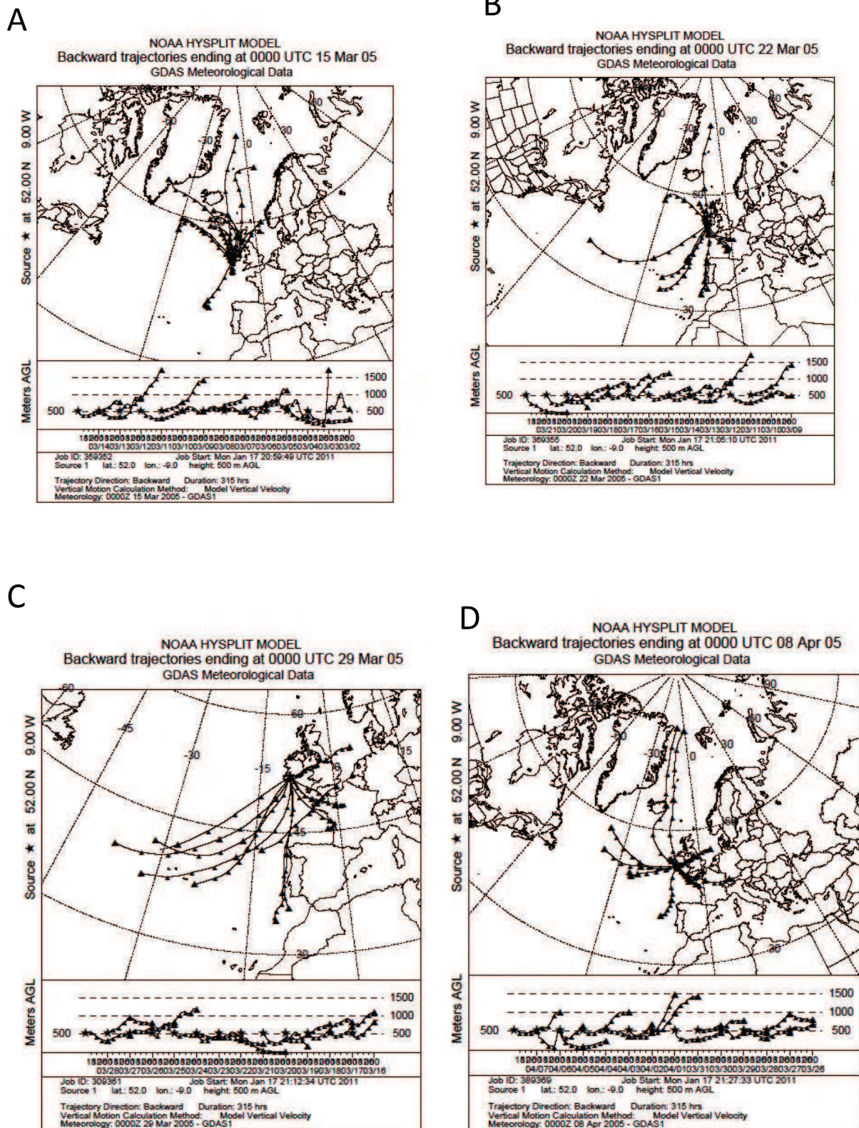
Fig. 2. Back trajectories of air mass flow over the observation site during study period obtained from NOAA HYSPLIT web based model; (A) March 15 th 2005; (B) March 22 nd 2005; (C) March 29 th 2005; (D) April 8 th 2005.
