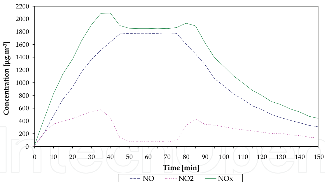
Fig. 6. Nitrogen oxides concentrations at a gas usage rate of 0.2 \text{ m}^3 \cdot \text{h}^{-1}
