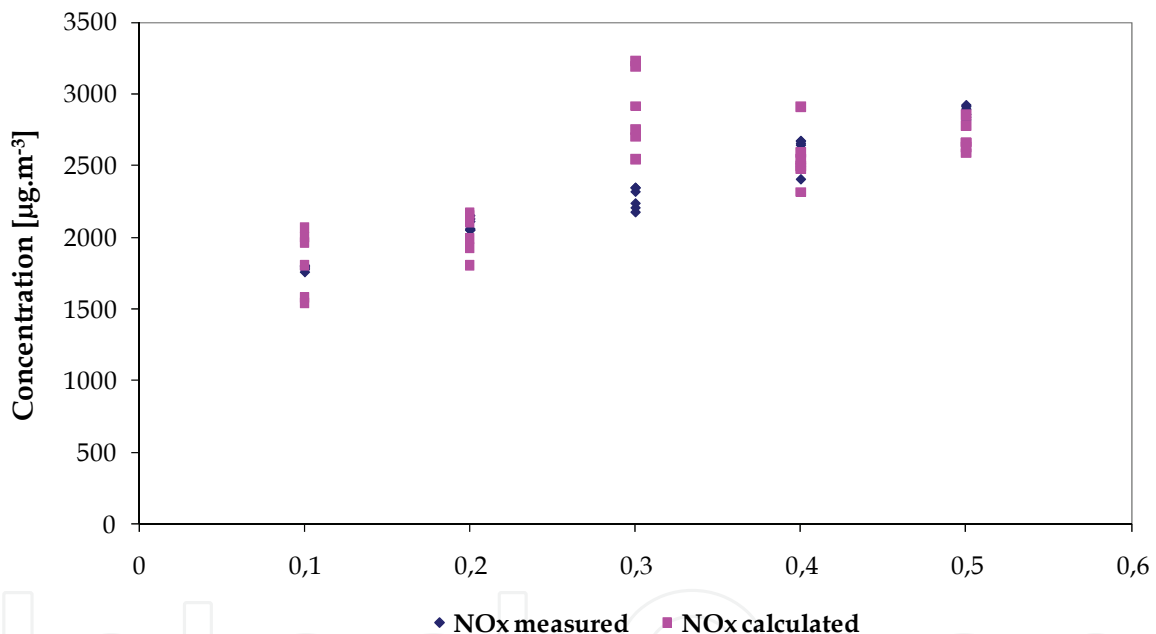
Fig. 7. Variance of measured and calculated \text{NO}_x concentrations for various gas intensities
