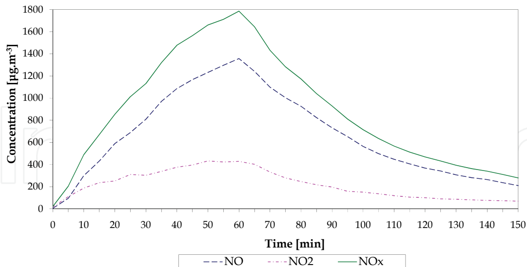
Fig. 5. Nitrogen oxides concentrations at a gas usage rate of 0.1 \text{ m}^3 \cdot \text{h}^{-1}
