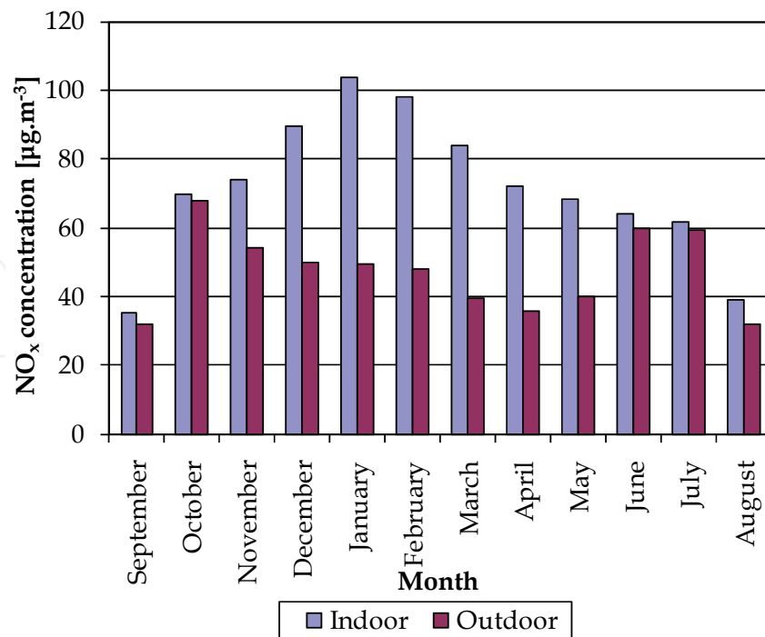
Fig. 1. Mean indoor and outdoor NO x concentrations throughout the year
