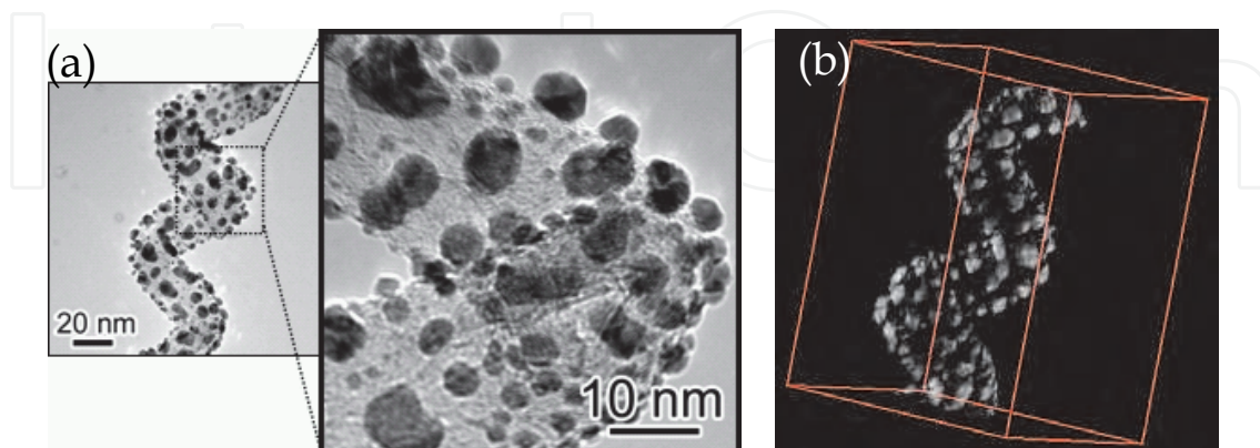
Fig. 26. Electron tomography of an MWCNC. (a) TEM micrograph of the MWCNC coated with Au nanoparticles. (b) Volume rendering image of the reconstructed MWCNC 3D image of (a). These images show that the MWCNC had a helical shape with a left-hand helix.
