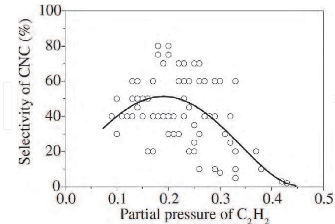
Fig. 8. Selectivity of CNCs plotted with partial pressure of \text{C}_2\text{H}_2 in a mixture with He gas. The process conditions are the same as those in the case of Fig. 7. (Xu et al., 2005)
