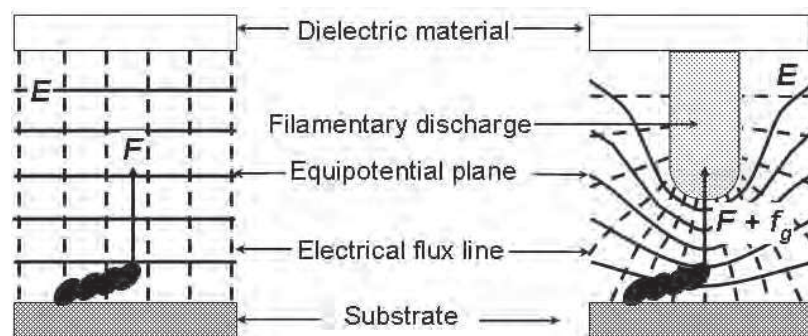
Fig. 31. Schematic illustrations of orientation force on CNTw: (a) uniform electric field in 'glow mode,' (b) non-uniform electric field in 'filament mode.' (Hosokawa et al., 2008)
