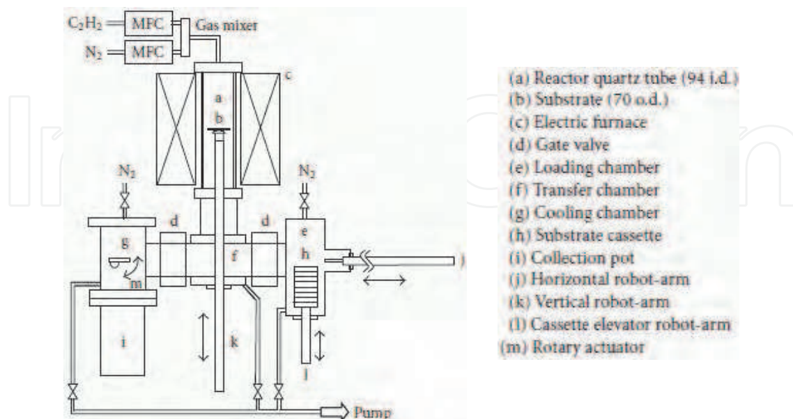
Fig. 2. Schematic diagram of automatic CVD system with a consecutive substrate transfer mechanism. (Hosokawa et al., 2007)
