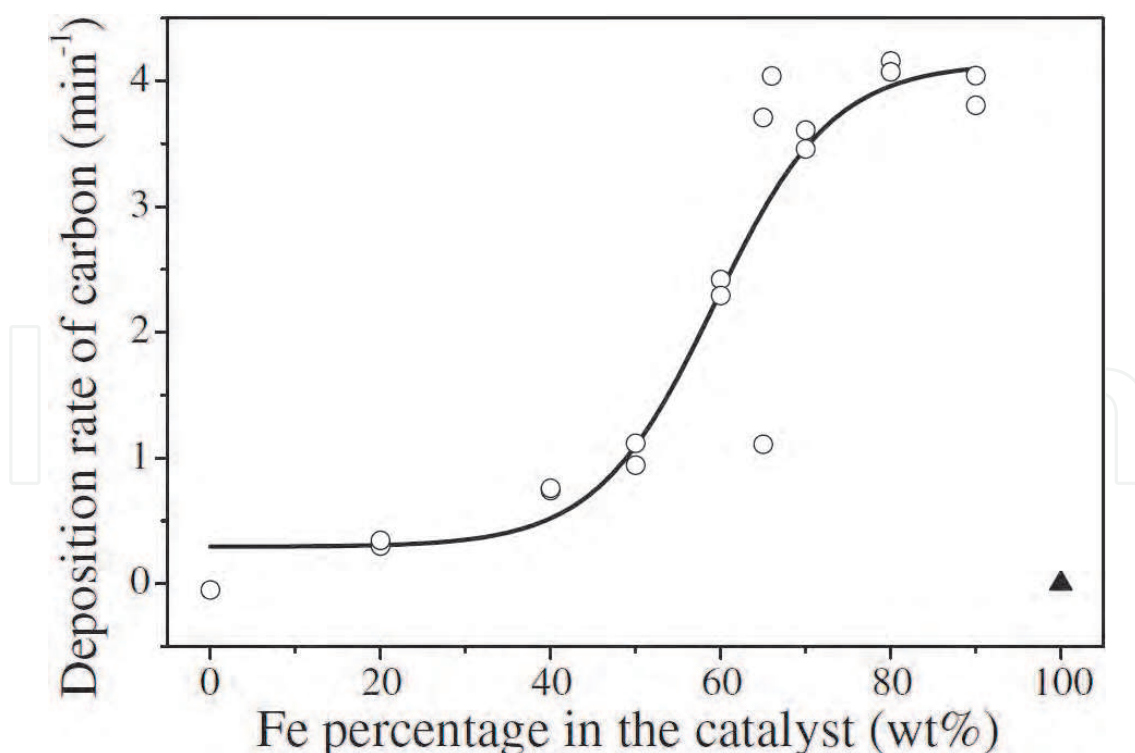
Fig. 3. Deposition rates of carbon materials on the composition of the catalyst. Pyrolysis of C 2 H 2 was carried out on 10 mg mixture of Fe and SnO 2 at 700°C for 10 min with the flow rates of C 2 H 2 and He gases of 180 and 420 ml/min, respectively. (Xu et al., 2005)
