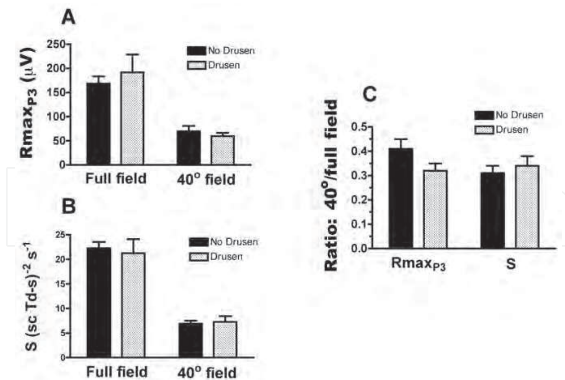
Fig. 3. Mean phototransduction parameters by drusen group. Mean rod maximal responses, R_{\text{maxP3}} (A) and sensitivities S (B) for drusen and no drusen monkeys for both full- and 40°-fields. C. Ratio of 40° to full field values for R_{\text{maxP3}} and S .
