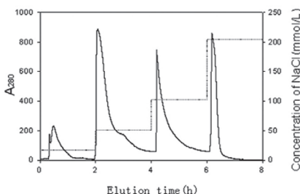
Fig. 5. Isolation of LF from the ultrafiltrated colostrum whey by an ion-exchange chromatography using DEAE-sepharose FF column ( 1.6 \times 75 cm). Adsorption phase, 500 mL ultra-filtrated colostrum whey (pH 6.8); washing phase, 300 mL de-ironed water; eluting phase, 600 mL 17 mmol/L, 600 mL 51 mmol/L, 600 mL 103 mmol/L, and 600 mL 205 mmol/L NaCl solution in a stepwise manner.
