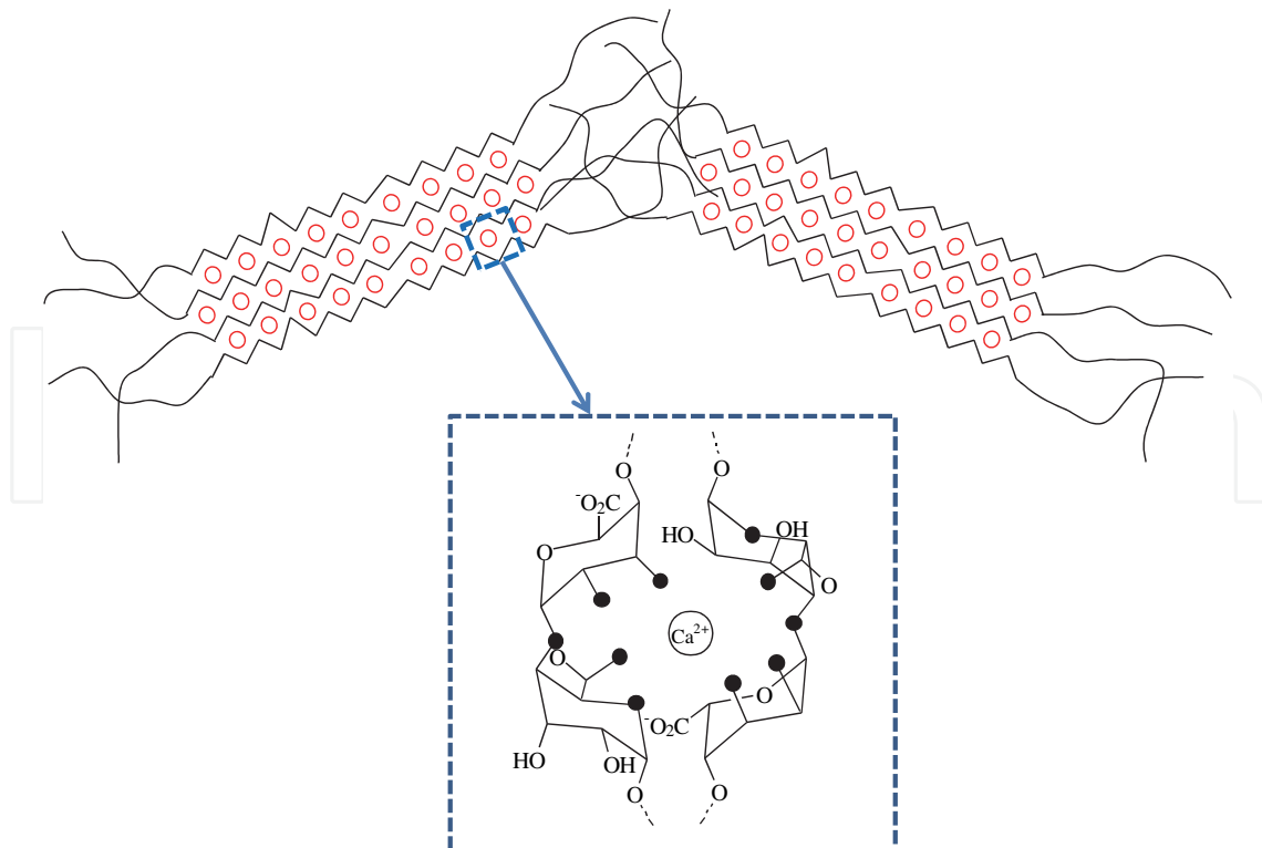
Fig. 4. Ionotropic gelation by interaction between anionic groups on alginate ( COO^- ) with divalent metal ions ( Ca^{2+} ).
