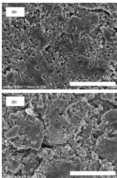
Fig. 2. SEM pictures of Fe-Cu-Si /C composite electrode annealed. Electrode --'a' at 110^\circ\text{C} and electrode ---'b' at 200^\circ\text{C} .
