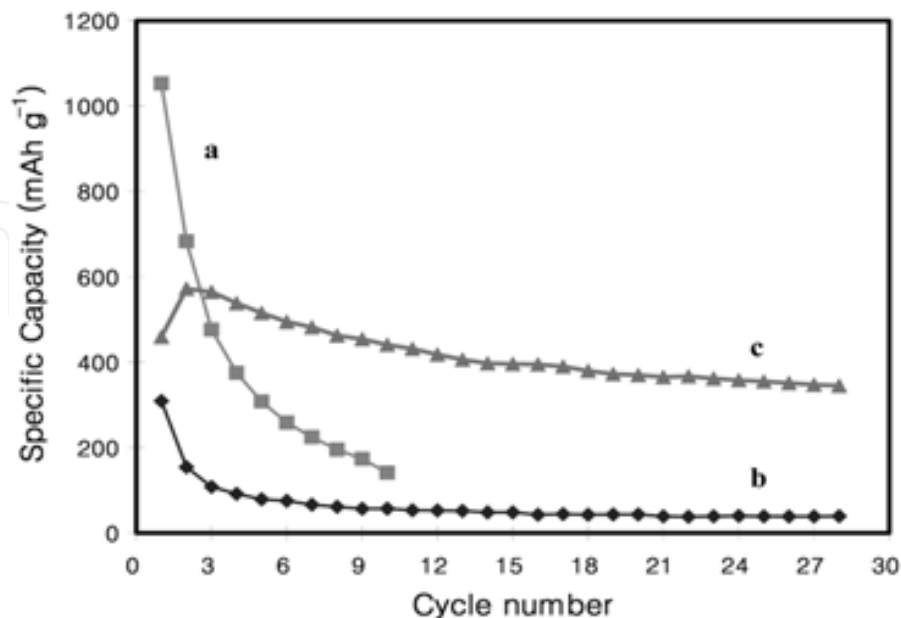
Fig. 19. Comparative delithiation behavior of a) Fe(1)Cu(1)Si(3.5) composite with Super 'P' black; b) Fe(1)Cu(1)Si(3.5)/Graphite ; c)Fe(1)Cu(1)Si(2.5)/Graphite.
