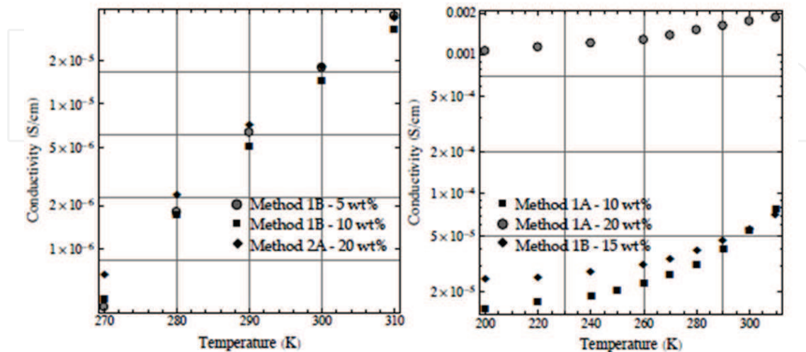
Fig. 12. Semi-log plots of conductivities of ionic conducting (left) and mixed conducting (right) polymer nanocomposite samples at various temperatures.
