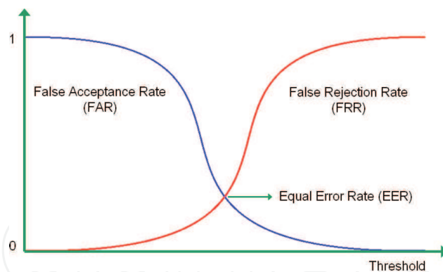
Fig. 4. EER as an intersection between FAR and FRR curves.
