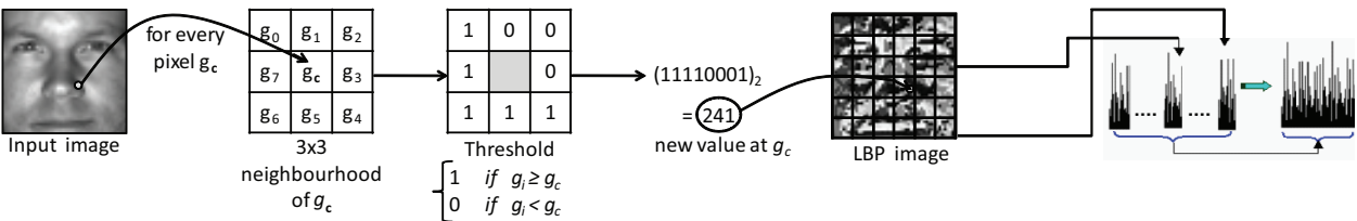
Fig. 2. Local Binary Patterns.
