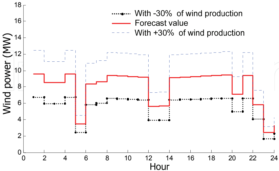
Fig. 18. Scenarios for wind power variation
