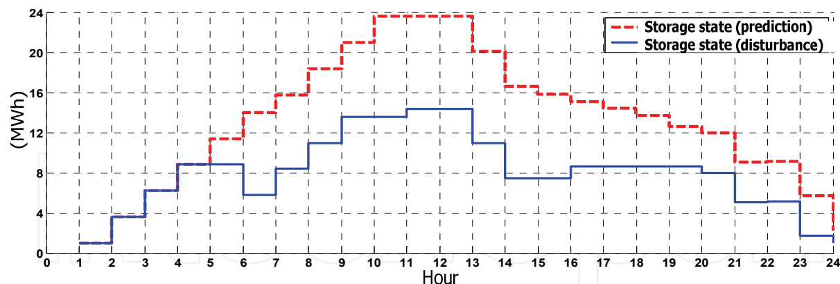
Fig. 23. Evolution of storage state
