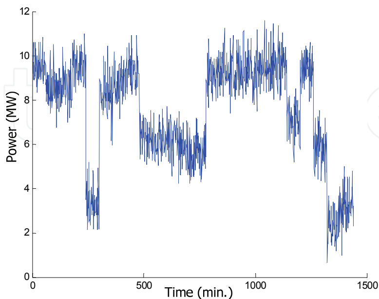
Fig. 6. Wind generation
