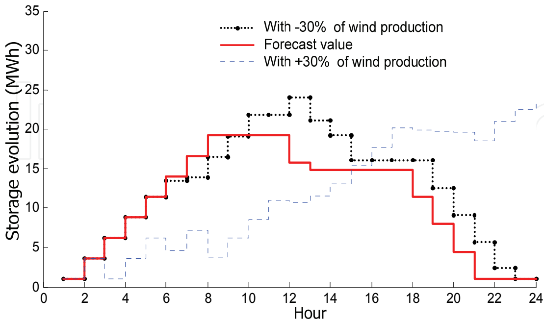
Fig. 19. Storage evolution in relation to produced wind power incertitude
