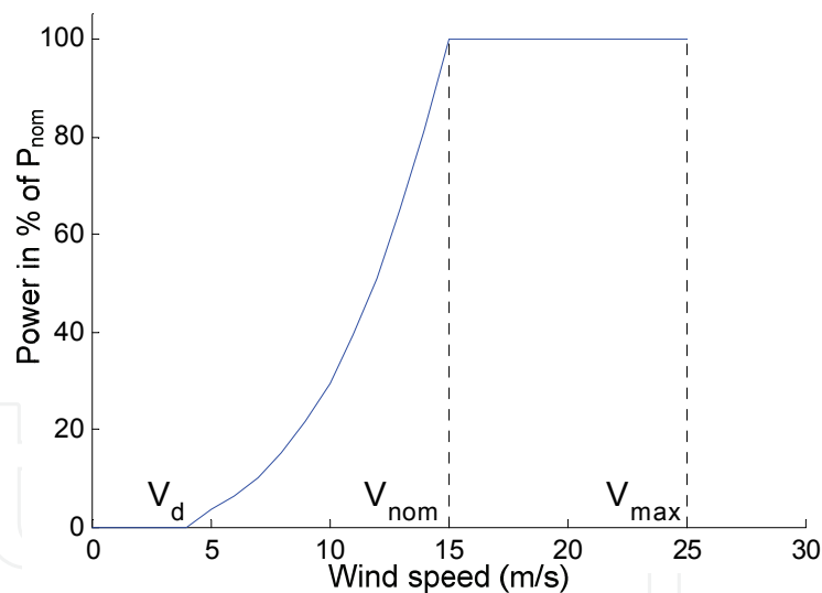
Fig. 3. Characteristic of the wind power according to the wind
