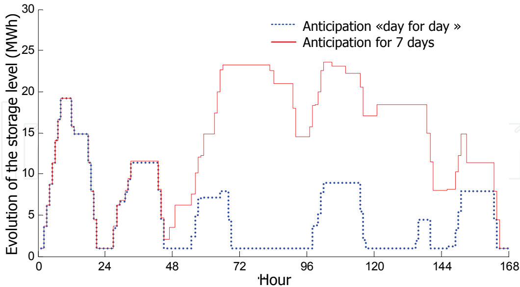
Fig. 15. Different strategies of storage management
