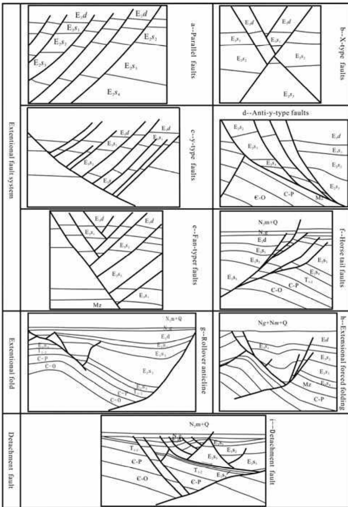
Fig. 12. Extensional tectonic styles in the Dongpu sag
