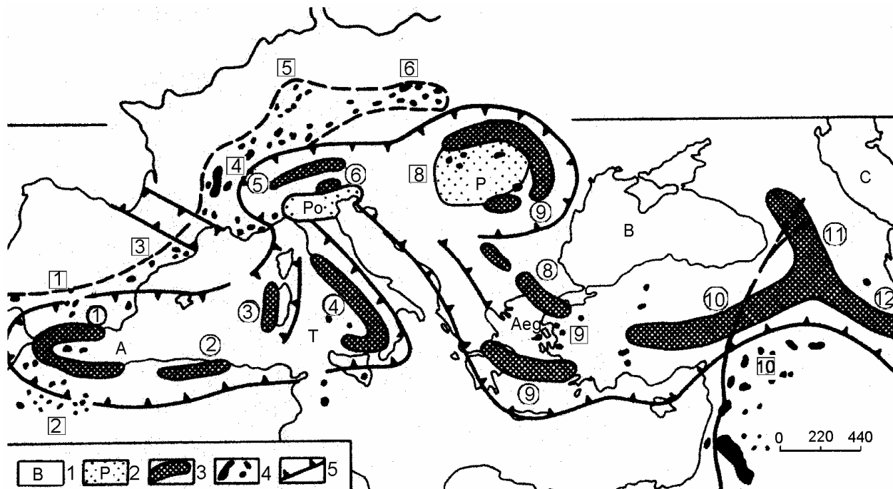
Fig. 5. Distribution of the late Cenozoic magmatism within the Alpine Belt 1 - back-arc seas (A - Alboran, T - Tyrrhenian; Ae - Aegian) and "downfall" seas (B - Black, C - Caspian); 2 - back-arc sedimentary basins (P- Pannonian, Po - Po valley); 3 - Late Cenozoic andesite-latitude volcanic arcs (in circles): 1 - Alboran, 2 - Cabil-Tell, 3 - Sardinian, 4 - South-Italian, 5 - Drava-Insubrian, 6 - Evganey, 7 - Carpatian, 8 - Balkanian, 9 - Aegian, 10-12 - Anatolia-Elbursian (10- Anatolia-Caucasian, 11 - zone of the Modern Caucasus volcanism, 12 - Caucasus-Elbursian); 4 - areas of flood basaltic volcanism (in square): 1 - South Spain and Portugal, 2 - Atlas, 3 - Eastern Spain, 4 - Central France massif, 5 - Rhine graben, 6 - Czech-Silesian, 7 - Pannonian, 8 - Western Turkey, 9 - northern Arabia; 5 - suture zones of major thrust structures
