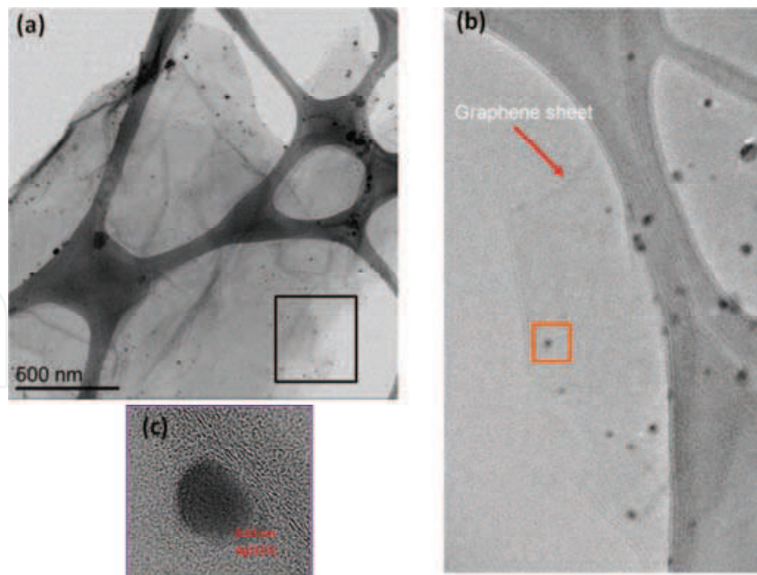
Fig. 12. (a) shows bright field TEM image of Ag/graphene sheet (b) HRTEM image of Ag/graphene sheet performed on the area denoted by black square region (a). (c) HR TEM image of single crystal Ag nanoparticle on graphene sheet which shows the characteristic (111) plane of Ag.
