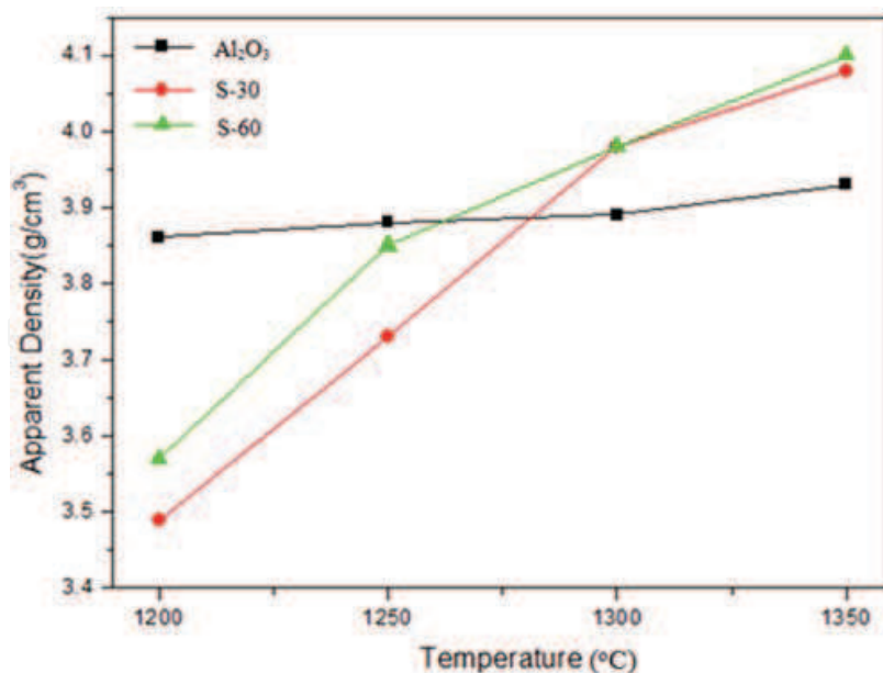
Fig. 22. The apparent density of the specimen of Al 2 O 3 , S-30, and S-60 prepared at a different SPS sintering temperature from 1200°C to 1350°C.
