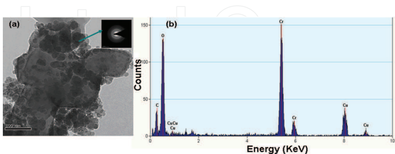
Fig. 5. TEM micrographs of (a) nanoparticles deposited on alumina particle (b) EDS spectrum of the coating particle.
