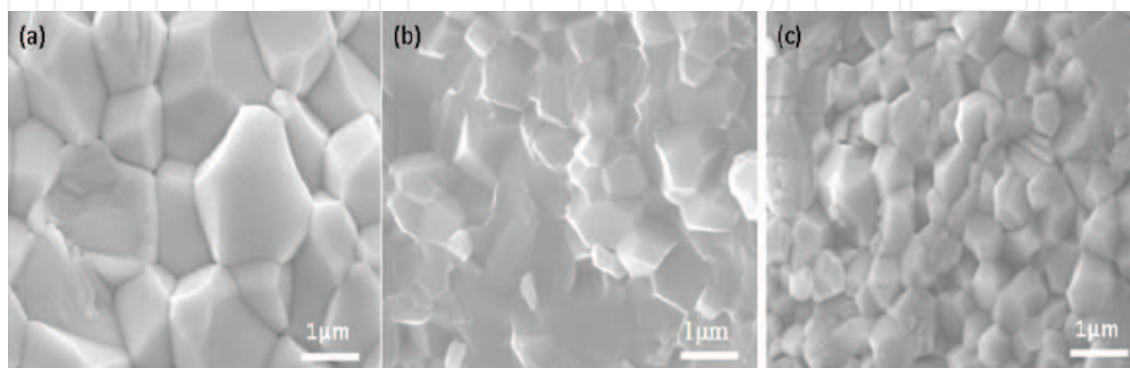
Fig. 23. SEM micrographs of fracture surface of 1350°C fully dense SPS specimen of (a) Al 2 O 3 , (b) S-30, (c) S-60.
