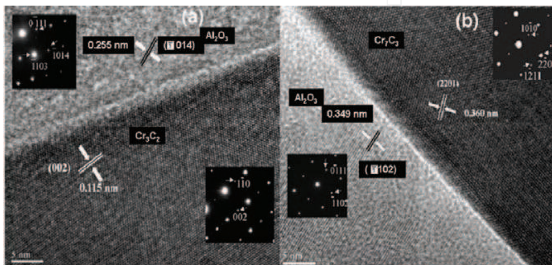
Fig. 9. Lattice images of the interfaces (a) between \text{Cr}_3\text{C}_2 and \text{Al}_2\text{O}_3 , and (b) between \text{Cr}_7\text{C}_3 and \text{Al}_2\text{O}_3 .
