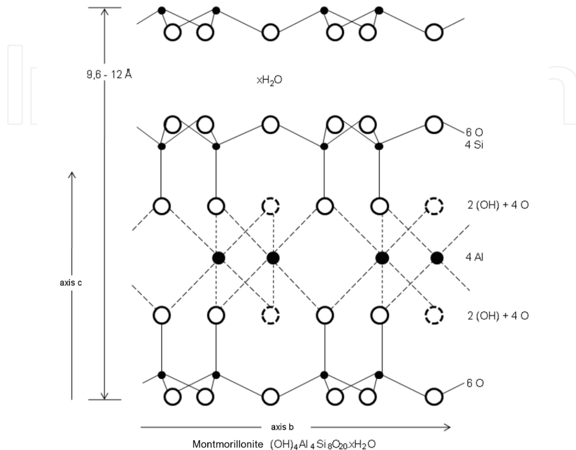
Fig. 1. Schematical representation of the montmorillonite structure (Papin, 1993).
