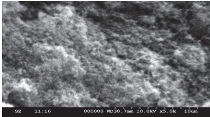
Fig. 1. d) Scanning electron micrograph (SEM) of MWCNT 2
