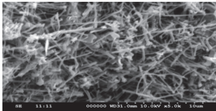
Fig. 1. b) Scanning Electron Micrograph (SEM) of MWCNT 1
