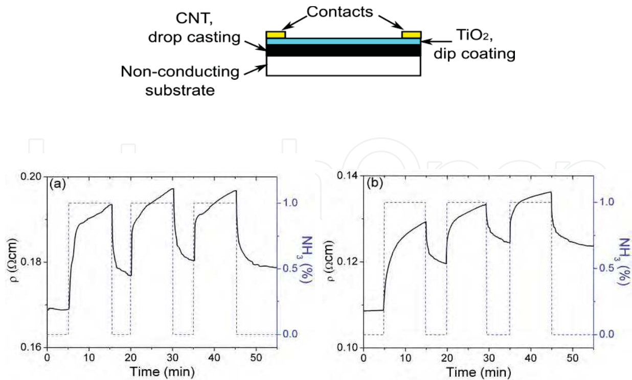
Fig. 9. Dynamical response to ammonia of compound films of CNTs (drop casting) and \text{TiO}_2 (dip coating): (a) CNT-WT/ \text{TiO}_2 ; (b) CNT-2.5/ \text{TiO}_2
