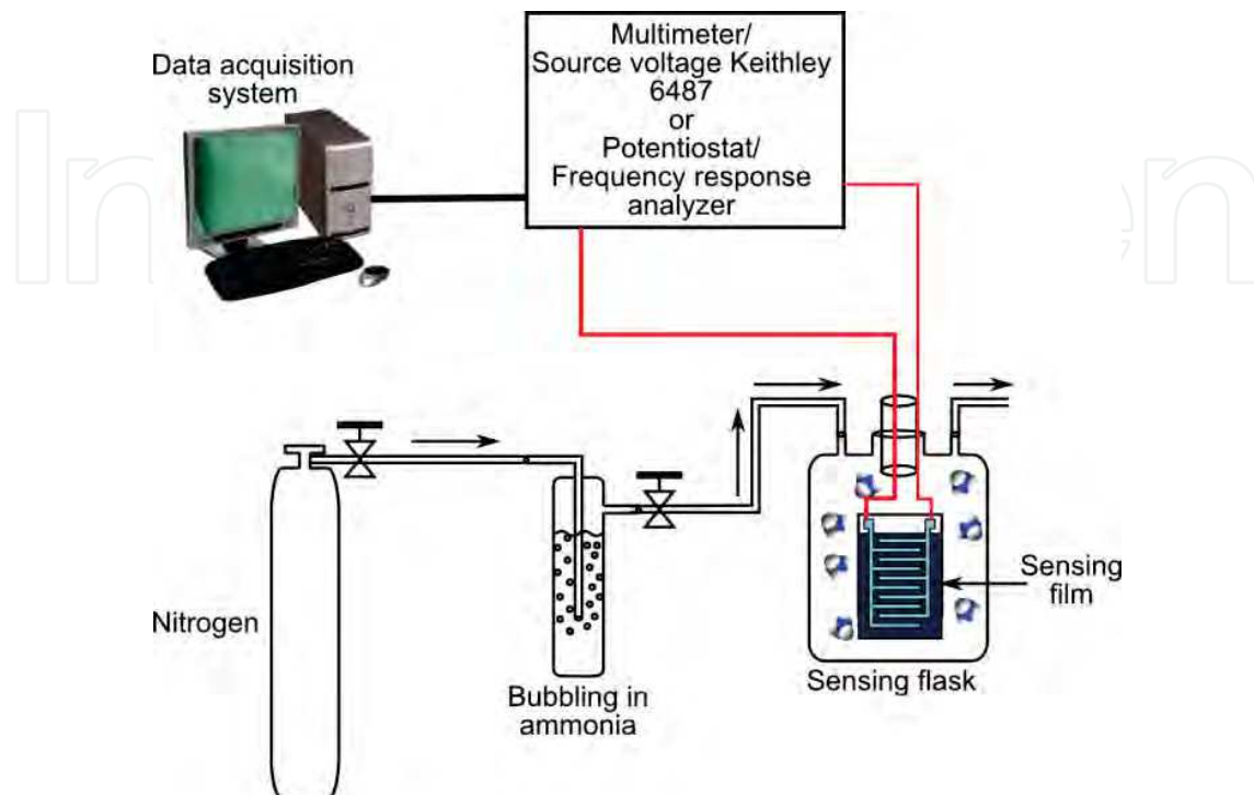
Fig. 1. Experimental setup used for sensing trials
