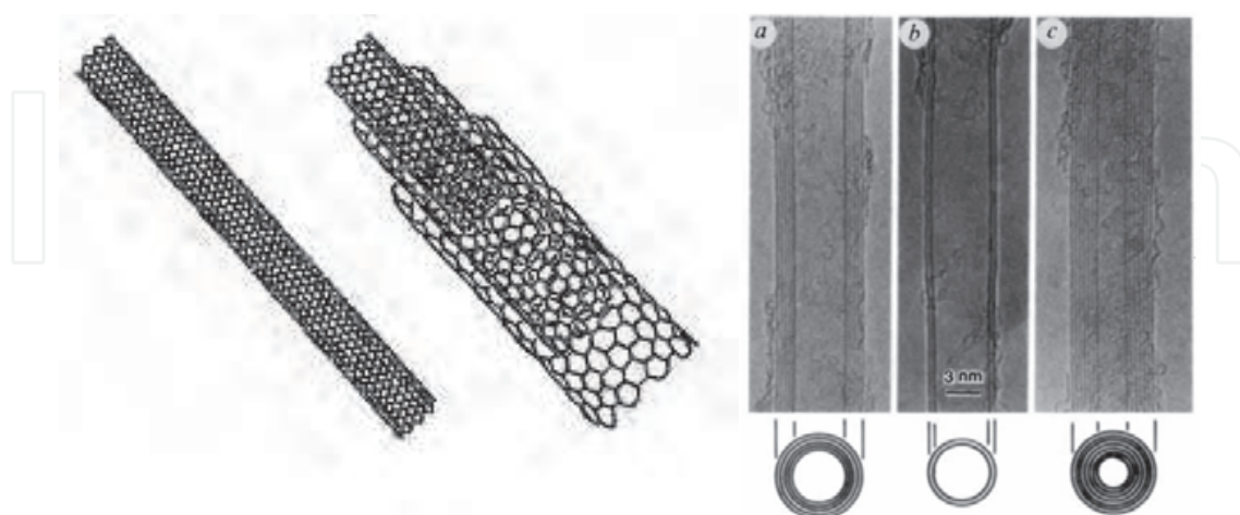
Fig. 1. Schematic of a SWCNT and MWNT (left). (Lacerda, Raffa, Prato, Bianco, & Kostarelos, 2007) and TEM of CNTs. a, Tube consisting of five graphitic sheets, diameter 6.7 nm. b, two-sheet, diameter 5.5 nm. c, seven-sheet, diameter 6.5 nm, which has the smallest hollow diameter (2.2 nm) (Iijima, 1991).
