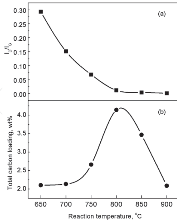
Fig. 6. Correlation diagram between synthesis temperatures ( ^{\circ}\text{C} ), quality index ( I_D/I_G ), and total carbon loading (%) (Chen, 2004b)
