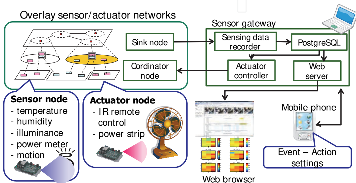
Fig. 6. Prototype implementation.
