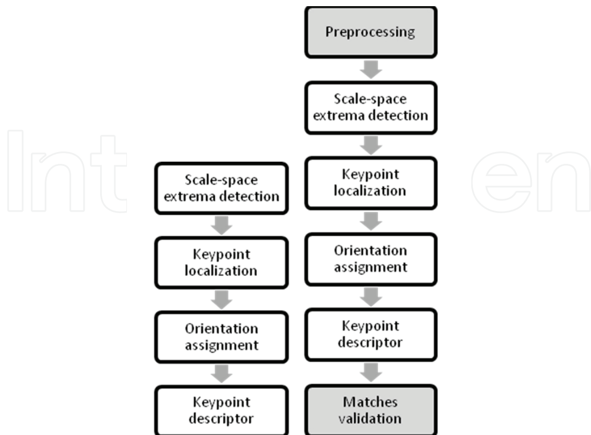
Fig. 12. On the Left the Lowe (Lowe, 2004) SIFT approach; on the right the contactless palmprint MSIFT approach proposed on this chapter.
