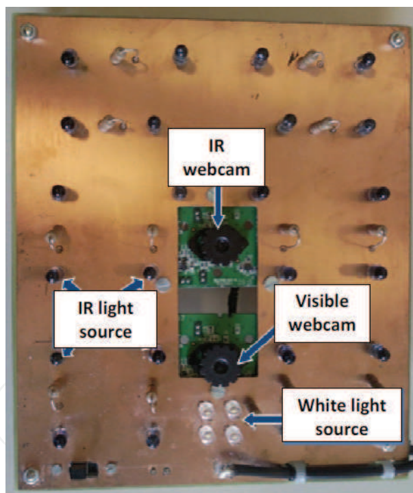
Fig. 2. Bispectral hand based biometric system
