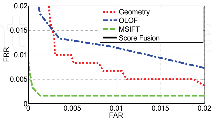
Fig. 15. DET curves of the proposed device. Dotted line: DET curve of geometrical device. Dash Dotted line: DET curve of OLOF features. Discontinuous line: DET curve of MSIFT features. Continuous line: DET curve of the combined scheme (OLOF+SIFT-Geometry).
