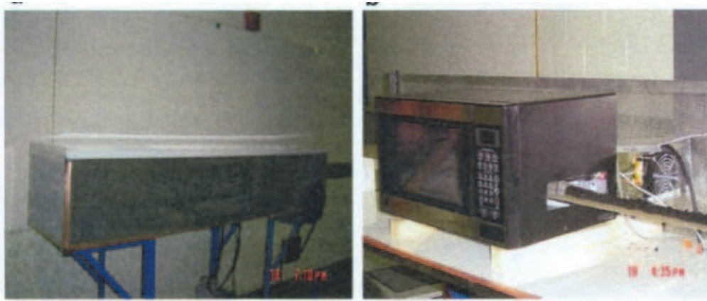
Fig. 5. (Left) Picture of the bench-scale microwave dewatering units with microwave shield in place. (Right) Close-up of the unit without the microwave shield showing the conveyor belt for feeding wet coal into the microwave oven (reproduced from the paper by Seehra et al., Fuel 2007).
