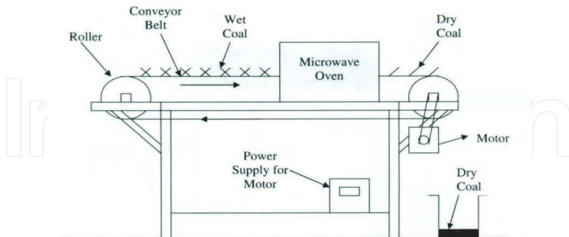
Fig. 4. Block diagram of the bench-scale microwave dewatering unit (reproduced from the paper by Seehra et al., Fuel 2007).
