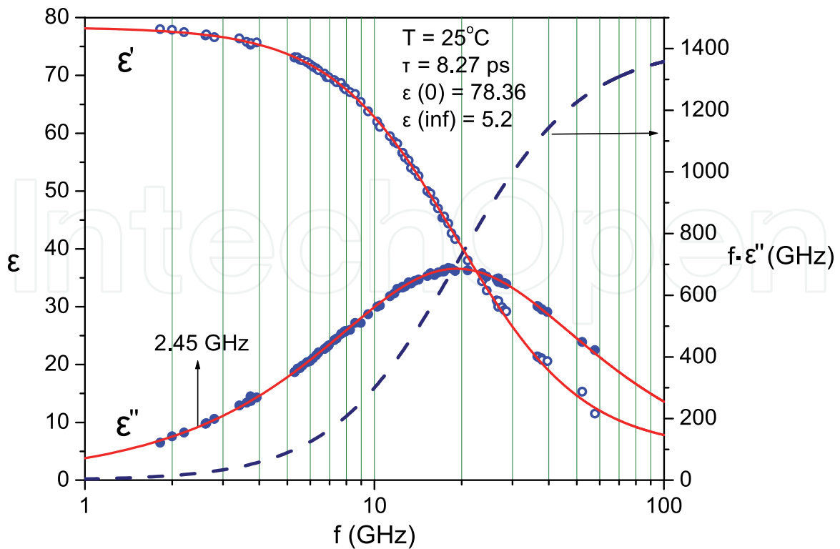
Fig. 1. The simulated plots of the frequency dependence of \epsilon' , \epsilon'' and f \cdot \epsilon'' for water using the data (circles) at 25°C from Kaatze (1989).
